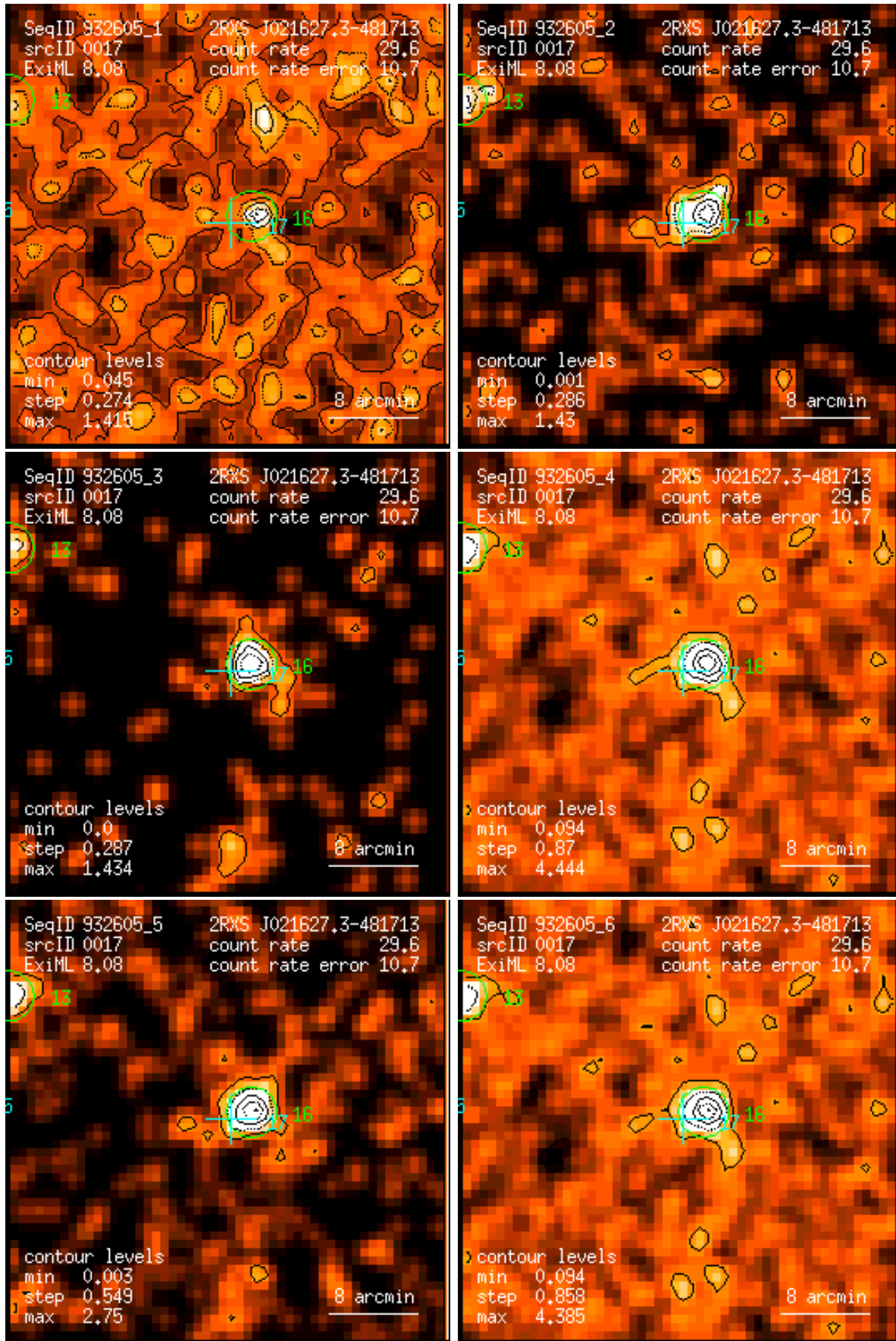
Figure 17: RASS 932605: detection 0017: band rate images, Gaussian filter: (1) PSPC channels 11 – 41, (2) 52 – 90, (3) 91 – 201, (4) 11 – 235, (5) 52 – 201, (6) 11 – 201. Broad band rates in counts/ks. Band rate contour levels in counts/ks/arcmin 2 .
