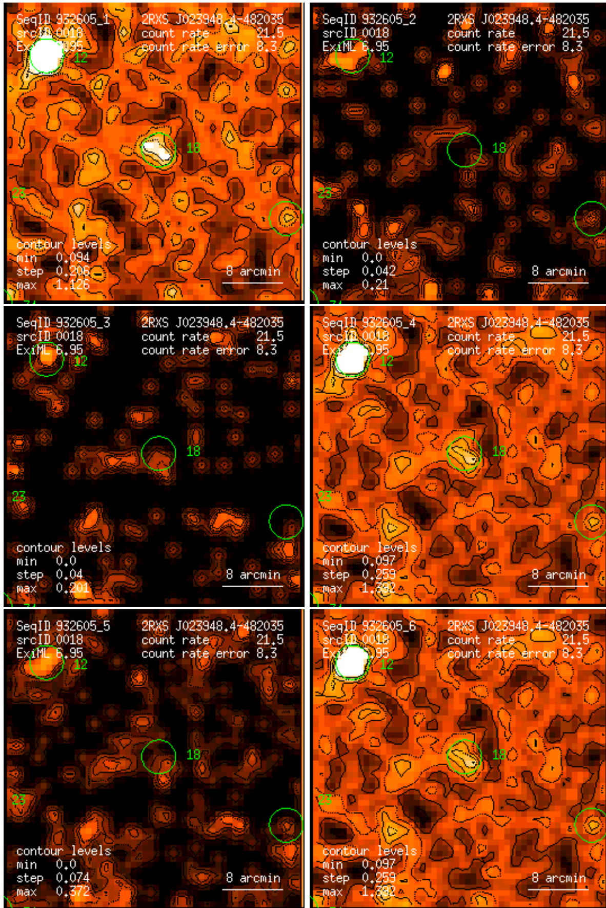
Figure 18: RASS 932605: detection 0018: band rate images, Gaussian filter: (1) PSPC channels 11 – 41, (2) 52 – 90, (3) 91 – 201, (4) 11 – 235, (5) 52 – 201, (6) 11 – 201. Broad band rates in counts/ks. Band rate contour levels in counts/ks/arcmin 2 .
