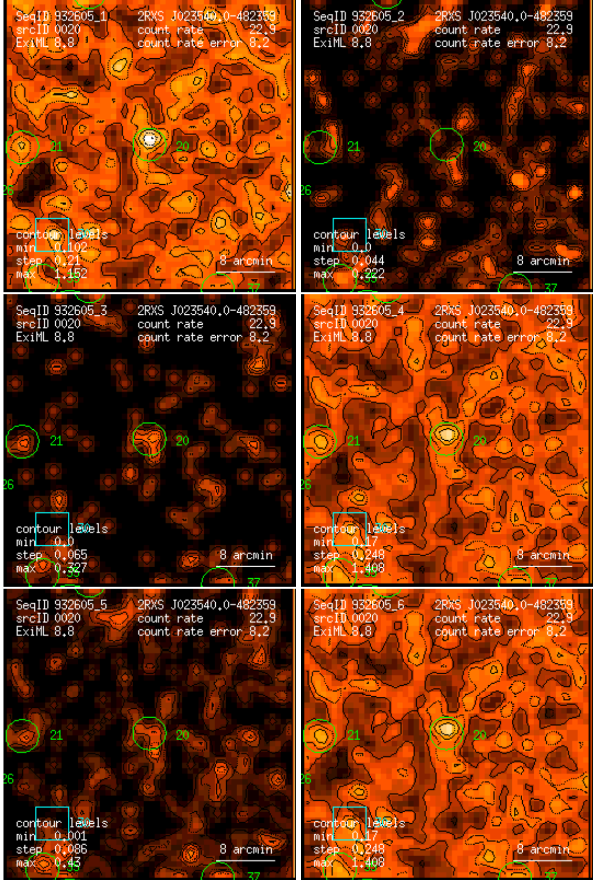
Figure 20: RASS 932605: detection 0020: band rate images, Gaussian filter: (1) PSPC channels 11 – 41, (2) 52 – 90, (3) 91 – 201, (4) 11 – 235, (5) 52 – 201, (6) 11 – 201. Broad band rates in counts/ks. Band rate contour levels in counts/ks/arcmin 2 .
