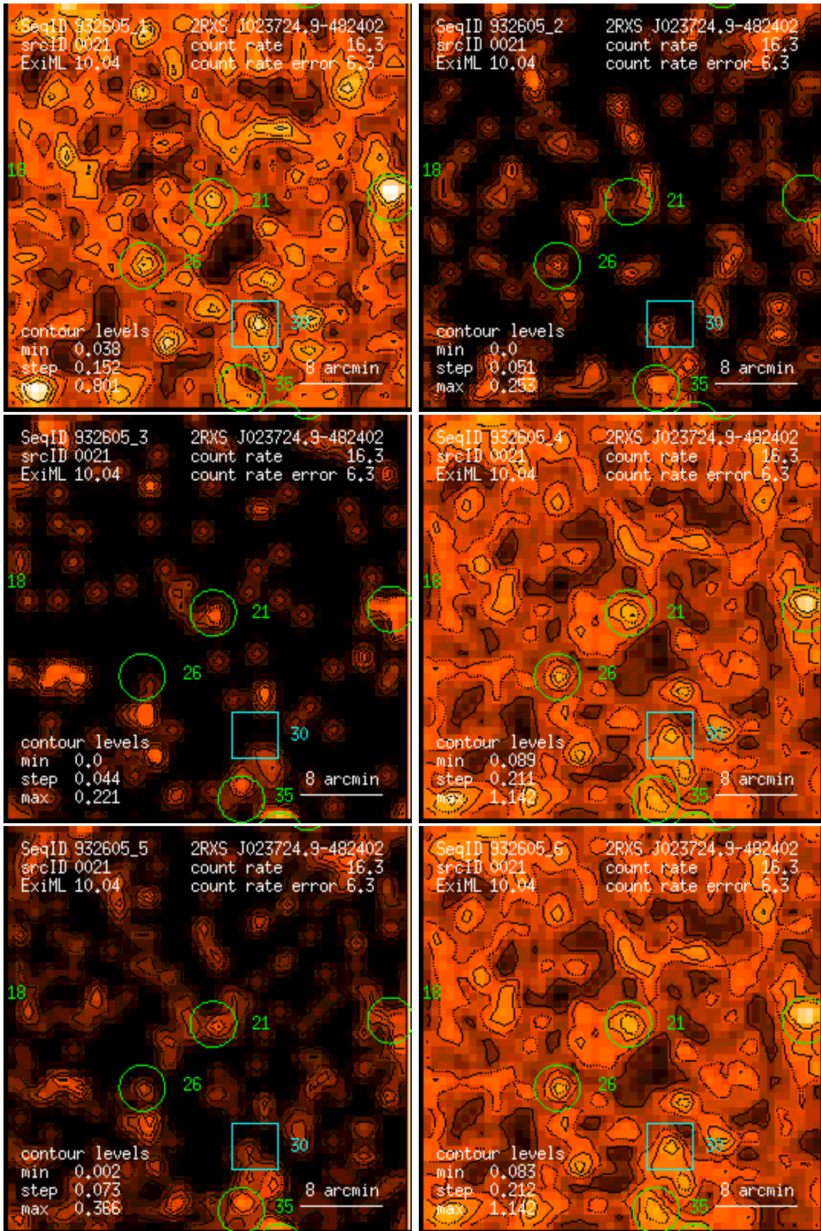
Figure 21: RASS 932605: detection 0021: band rate images, Gaussian filter: (1) PSPC channels 11 – 41, (2) 52 – 90, (3) 91 – 201, (4) 11 – 235, (5) 52 – 201, (6) 11 – 201. Broad band rates in counts/ks. Band rate contour levels in counts/ks/arcmin 2 .
