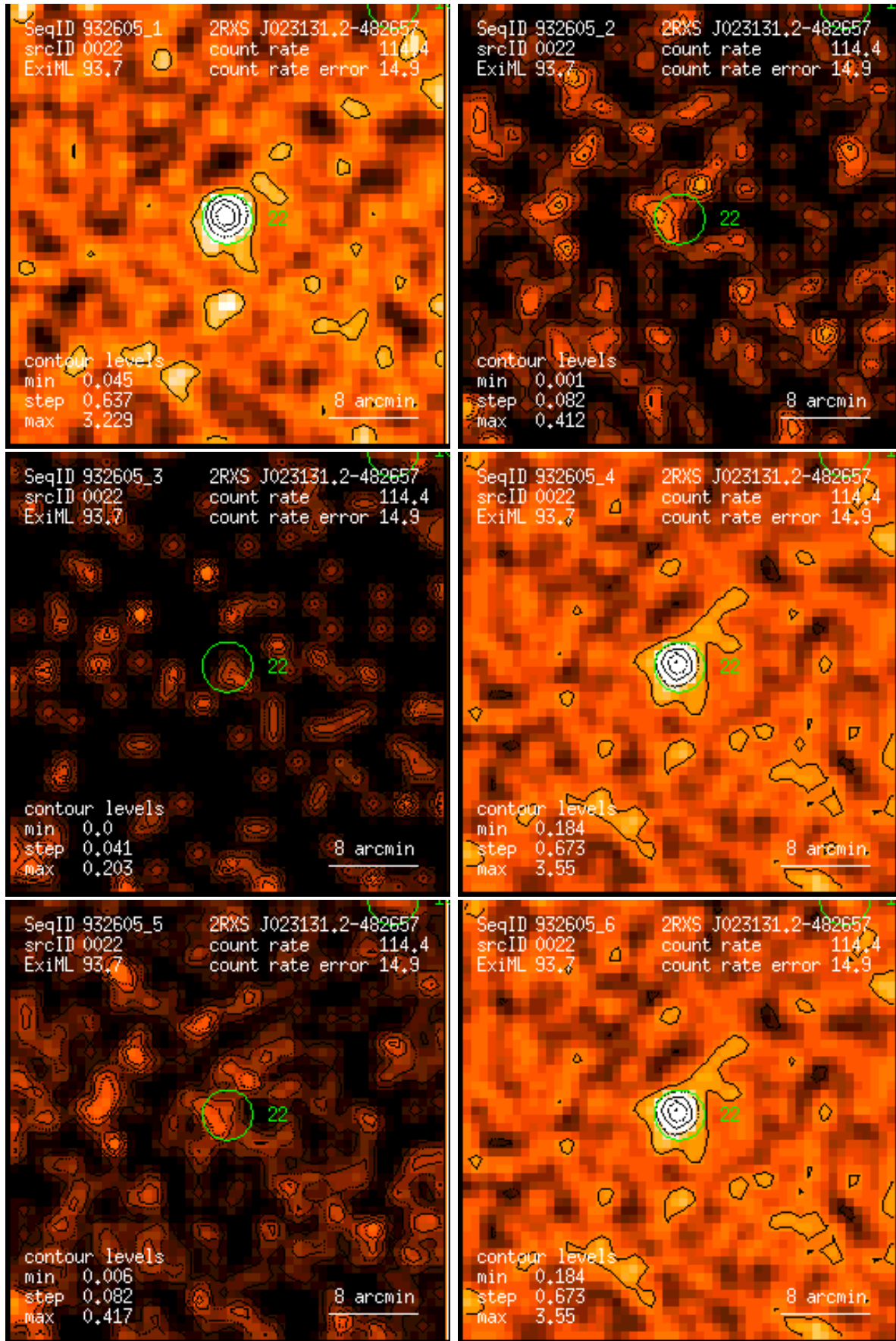
Figure 22: RASS 932605: detection 0022: band rate images, Gaussian filter: (1) PSPC channels 11 – 41, (2) 52 – 90, (3) 91 – 201, (4) 11 – 235, (5) 52 – 201, (6) 11 – 201. Broad band rates in counts/ks. Band rate contour levels in counts/ks/arcmin 2 .
