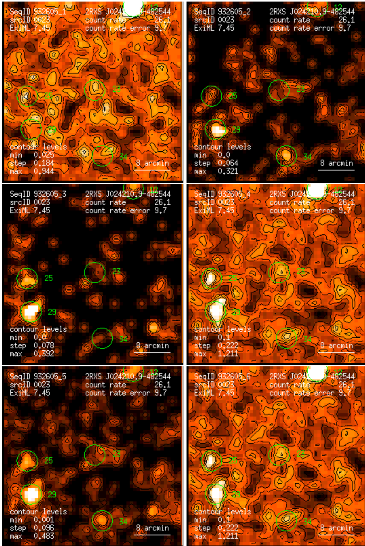
Figure 23: RASS 932605: detection 0023: band rate images, Gaussian filter: (1) PSPC channels 11 – 41, (2) 52 – 90, (3) 91 – 201, (4) 11 – 235, (5) 52 – 201, (6) 11 – 201. Broad band rates in counts/ks. Band rate contour levels in counts/ks/arcmin 2 .
