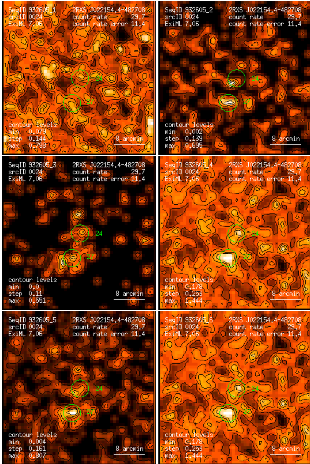
Figure 24: RASS 932605: detection 0024: band rate images, Gaussian filter: (1) PSPC channels 11 – 41, (2) 52 – 90, (3) 91 – 201, (4) 11 – 235, (5) 52 – 201, (6) 11 – 201. Broad band rates in counts/ks. Band rate contour levels in counts/ks/arcmin 2 .
