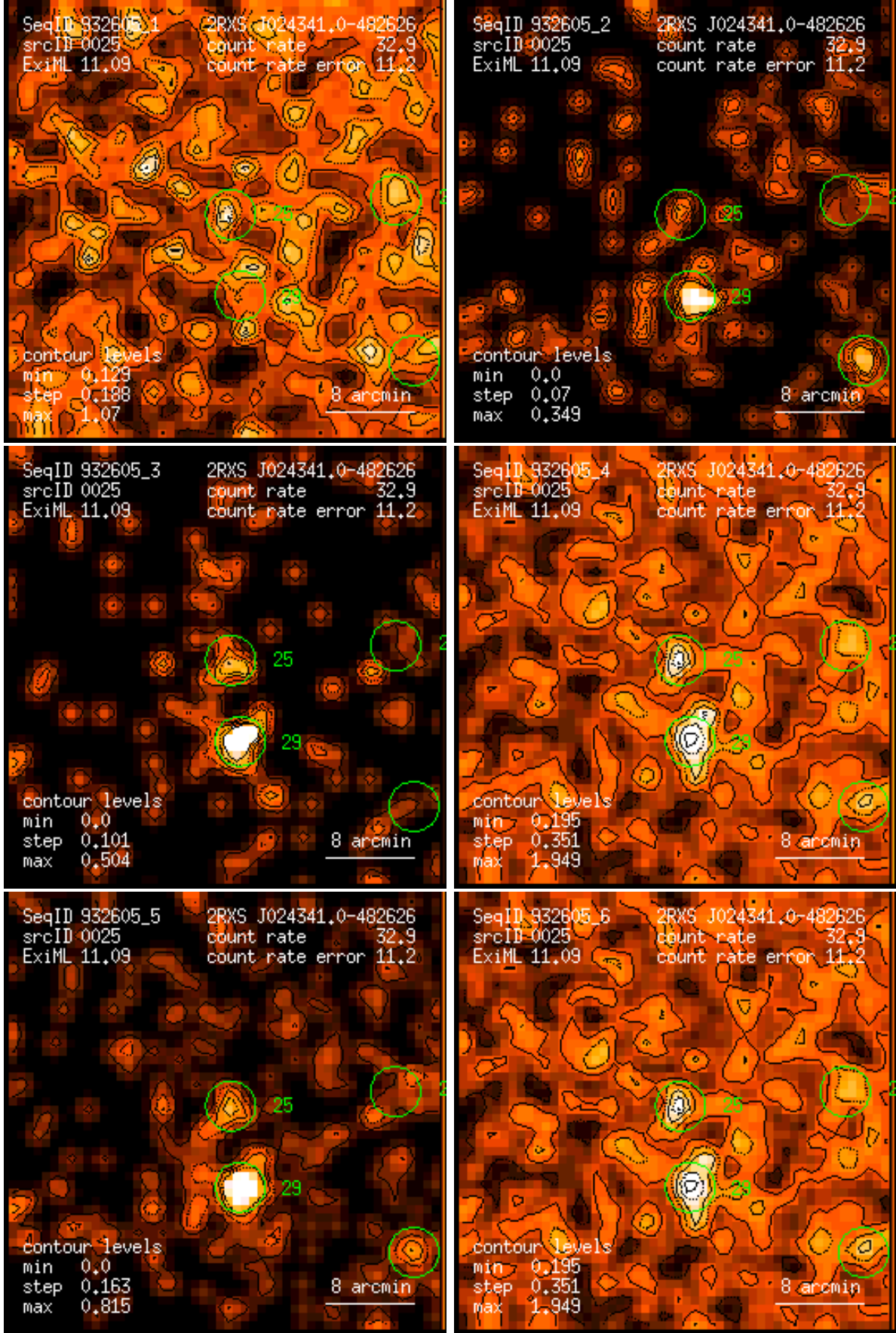
Figure 25: RASS 932605: detection 0025: band rate images, Gaussian filter: (1) PSPC channels 11 – 41, (2) 52 – 90, (3) 91 – 201, (4) 11 – 235, (5) 52 – 201, (6) 11 – 201. Broad band rates in counts/ks. Band rate contour levels in counts/ks/arcmin 2 .
