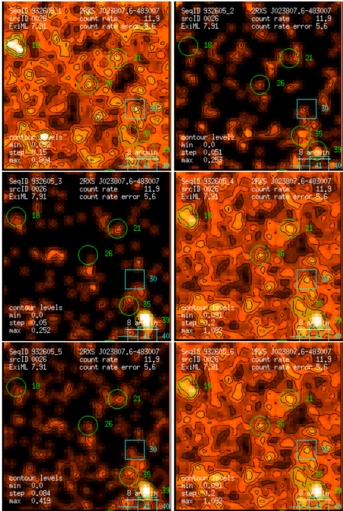
Figure 26: RASS 932605: detection 0026: band rate images, Gaussian filter: (1) PSPC channels 11 – 41, (2) 52 – 90, (3) 91 – 201, (4) 11 – 235, (5) 52 – 201, (6) 11 – 201. Broad band rates in counts/ks. Band rate contour levels in counts/ks/arcmin 2 .
