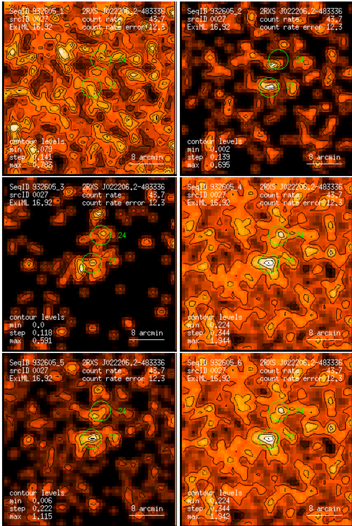
Figure 27: RASS 932605: detection 0027: band rate images, Gaussian filter: (1) PSPC channels 11 – 41, (2) 52 – 90, (3) 91 – 201, (4) 11 – 235, (5) 52 – 201, (6) 11 – 201. Broad band rates in counts/ks. Band rate contour levels in counts/ks/arcmin 2 .
