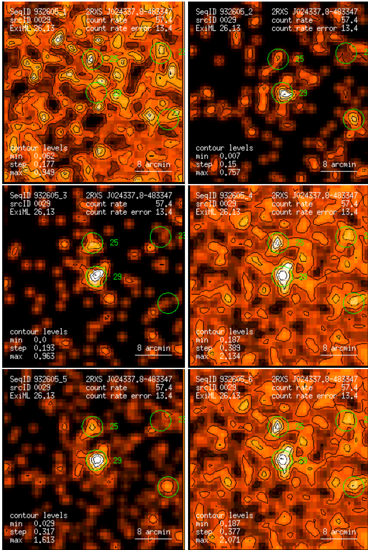
Figure 29: RASS 932605: detection 0029: band rate images, Gaussian filter: (1) PSPC channels 11 – 41, (2) 52 – 90, (3) 91 – 201, (4) 11 – 235, (5) 52 – 201, (6) 11 – 201. Broad band rates in counts/ks. Band rate contour levels in counts/ks/arcmin 2 .
