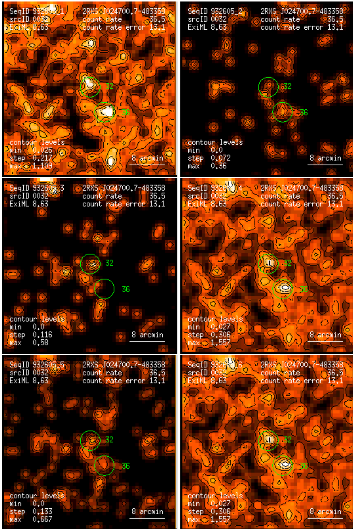
Figure 32: RASS 932605: detection 0032: band rate images, Gaussian filter: (1) PSPC channels 11 – 41, (2) 52 – 90, (3) 91 – 201, (4) 11 – 235, (5) 52 – 201, (6) 11 – 201. Broad band rates in counts/ks. Band rate contour levels in counts/ks/arcmin 2 .
