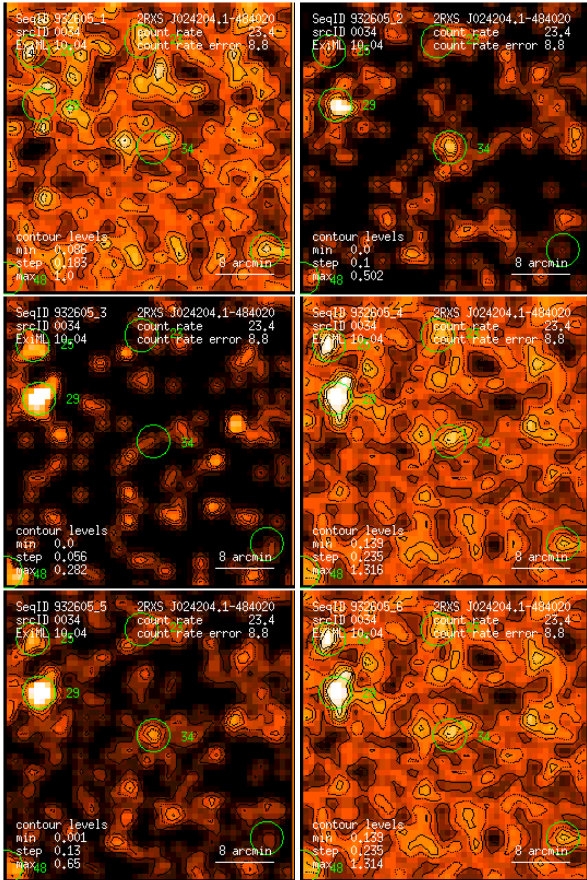
Figure 34: RASS 932605: detection 0034: band rate images, Gaussian filter: (1) PSPC channels 11 – 41, (2) 52 – 90, (3) 91 – 201, (4) 11 – 235, (5) 52 – 201, (6) 11 – 201. Broad band rates in counts/ks. Band rate contour levels in counts/ks/arcmin 2 .
