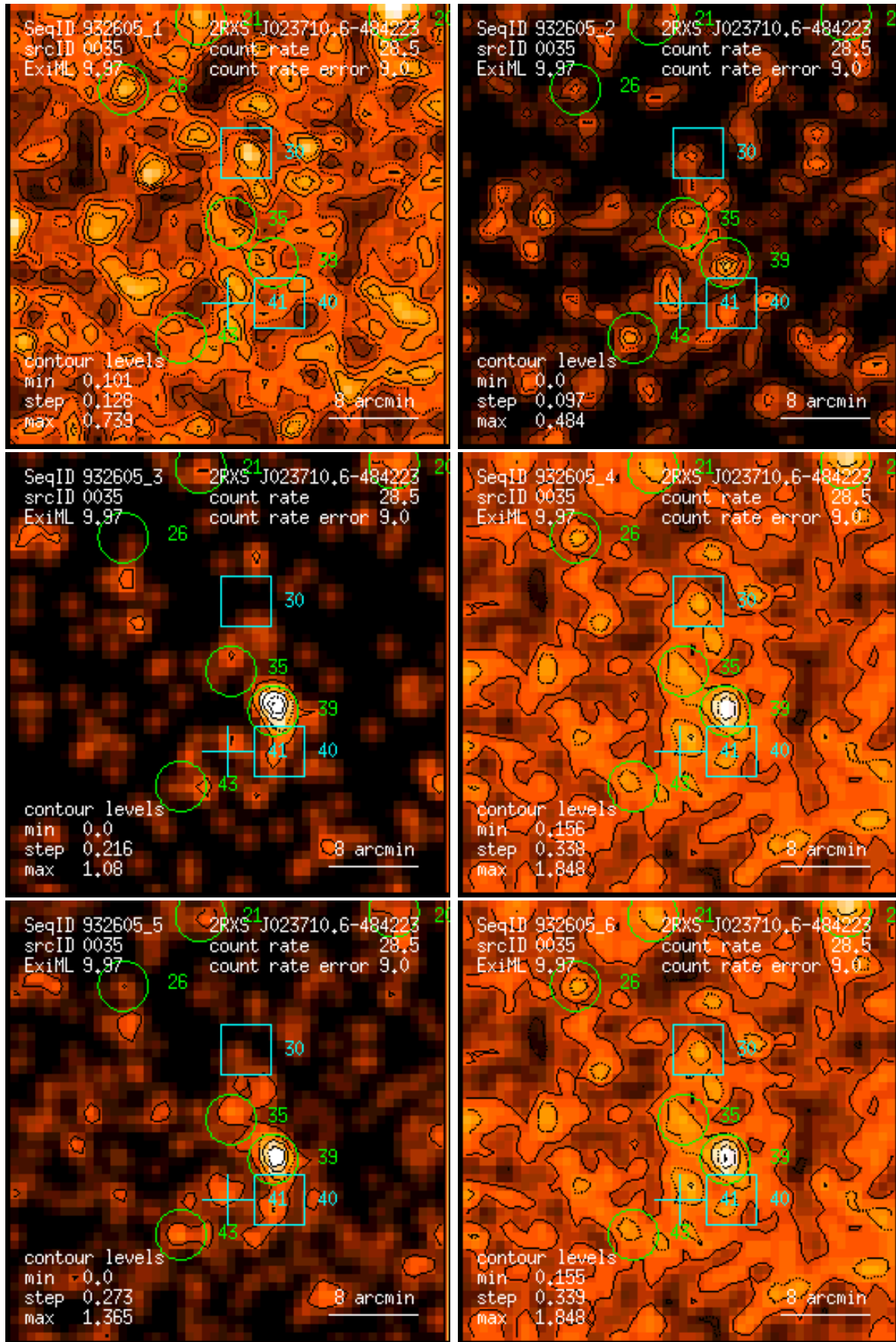
Figure 35: RASS 932605: detection 0035: band rate images, Gaussian filter: (1) PSPC channels 11 – 41, (2) 52 – 90, (3) 91 – 201, (4) 11 – 235, (5) 52 – 201, (6) 11 – 201. Broad band rates in counts/ks. Band rate contour levels in counts/ks/arcmin 2 .
