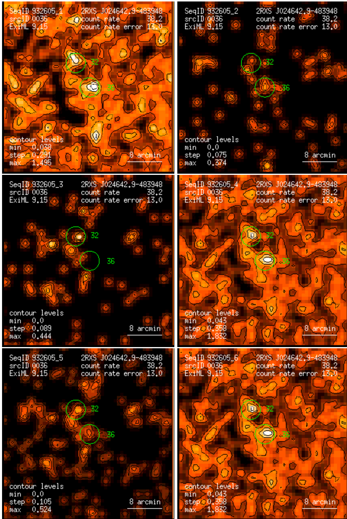
Figure 36: RASS 932605: detection 0036: band rate images, Gaussian filter: (1) PSPC channels 11 – 41, (2) 52 – 90, (3) 91 – 201, (4) 11 – 235, (5) 52 – 201, (6) 11 – 201. Broad band rates in counts/ks. Band rate contour levels in counts/ks/arcmin 2 .
