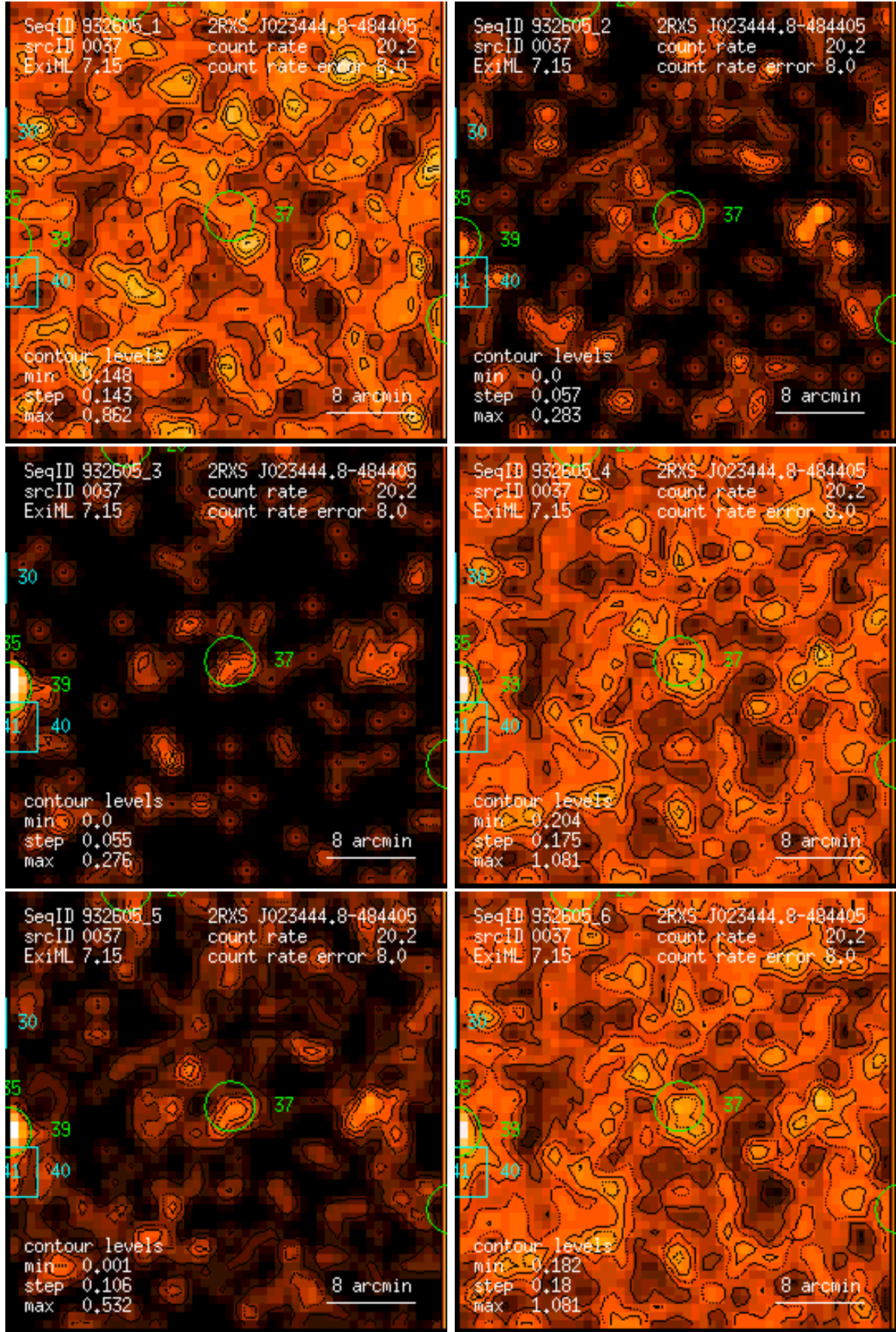
Figure 37: RASS 932605: detection 0037: band rate images, Gaussian filter: (1) PSPC channels 11 – 41, (2) 52 – 90, (3) 91 – 201, (4) 11 – 235, (5) 52 – 201, (6) 11 – 201. Broad band rates in counts/ks. Band rate contour levels in counts/ks/arcmin 2 .
