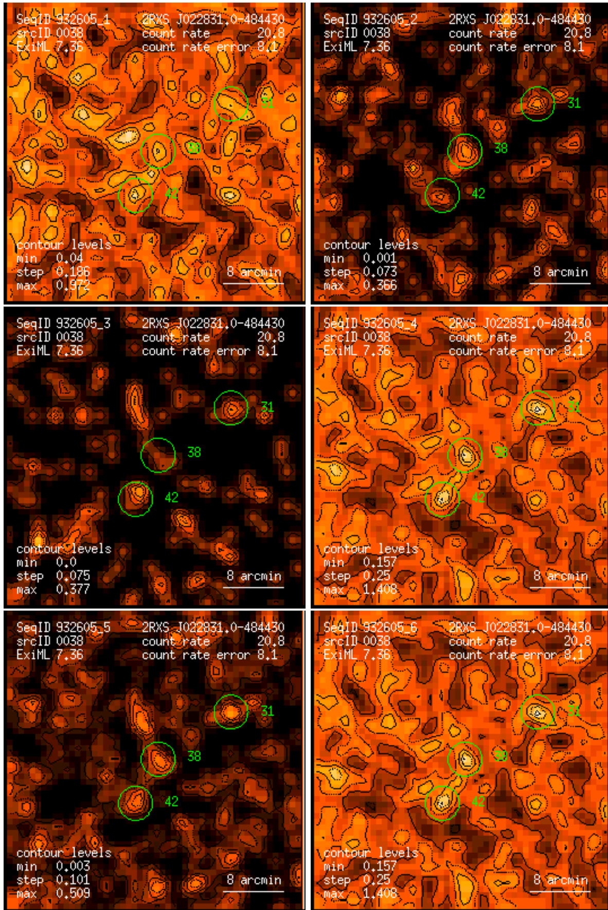
Figure 38: RASS 932605: detection 0038: band rate images, Gaussian filter: (1) PSPC channels 11 – 41, (2) 52 – 90, (3) 91 – 201, (4) 11 – 235, (5) 52 – 201, (6) 11 – 201. Broad band rates in counts/ks. Band rate contour levels in counts/ks/arcmin 2 .
