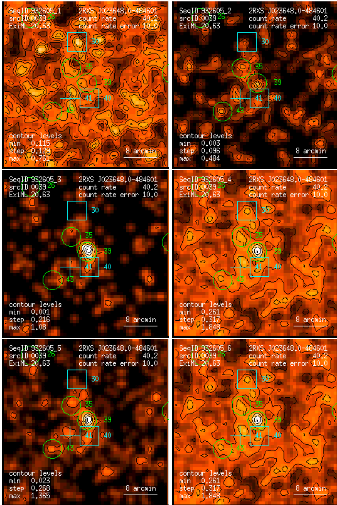
Figure 39: RASS 932605: detection 0039: band rate images, Gaussian filter: (1) PSPC channels 11 – 41, (2) 52 – 90, (3) 91 – 201, (4) 11 – 235, (5) 52 – 201, (6) 11 – 201. Broad band rates in counts/ks. Band rate contour levels in counts/ks/arcmin 2 .
