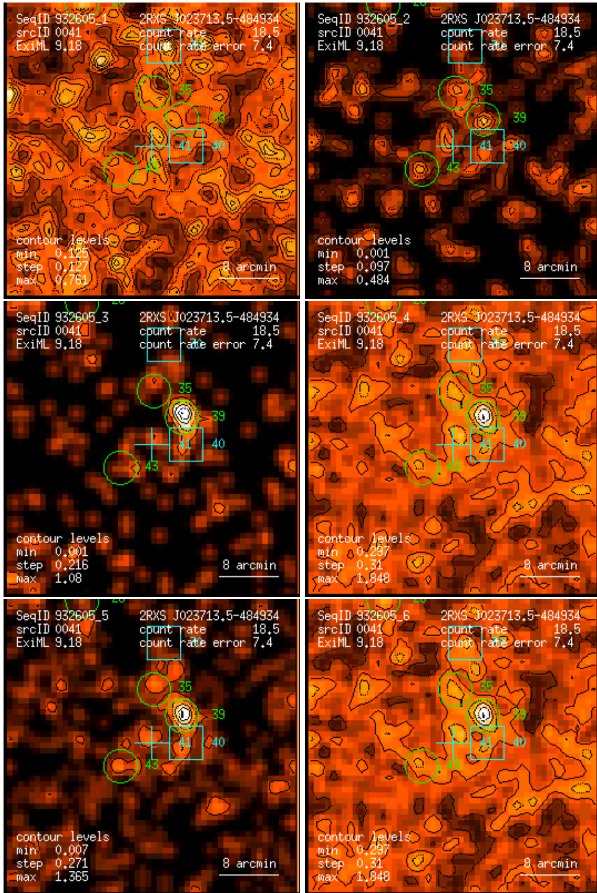
Figure 41: RASS 932605: detection 0041: band rate images, Gaussian filter: (1) PSPC channels 11 – 41, (2) 52 – 90, (3) 91 – 201, (4) 11 – 235, (5) 52 – 201, (6) 11 – 201. Broad band rates in counts/ks. Band rate contour levels in counts/ks/arcmin 2 .
