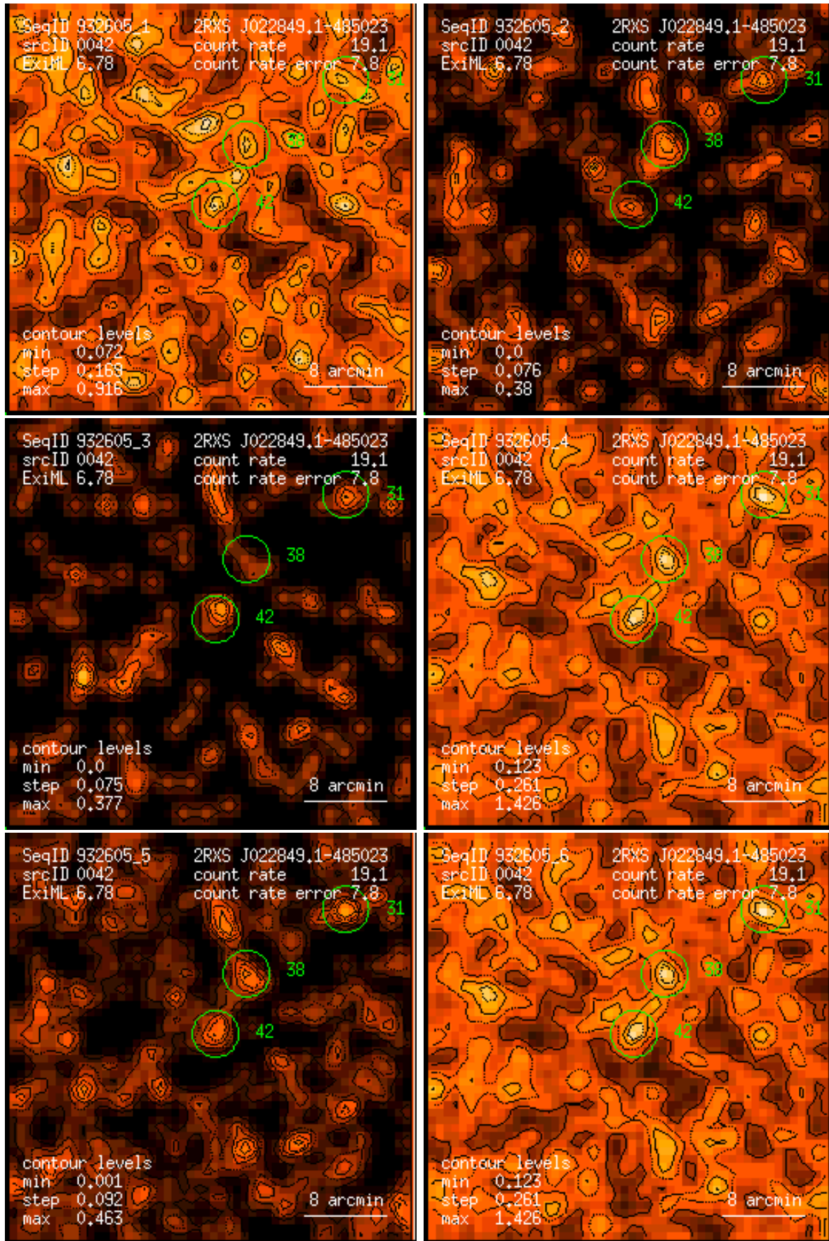
Figure 42: RASS 932605: detection 0042: band rate images, Gaussian filter: (1) PSPC channels 11 – 41, (2) 52 – 90, (3) 91 – 201, (4) 11 – 235, (5) 52 – 201, (6) 11 – 201. Broad band rates in counts/ks. Band rate contour levels in counts/ks/arcmin 2 .
