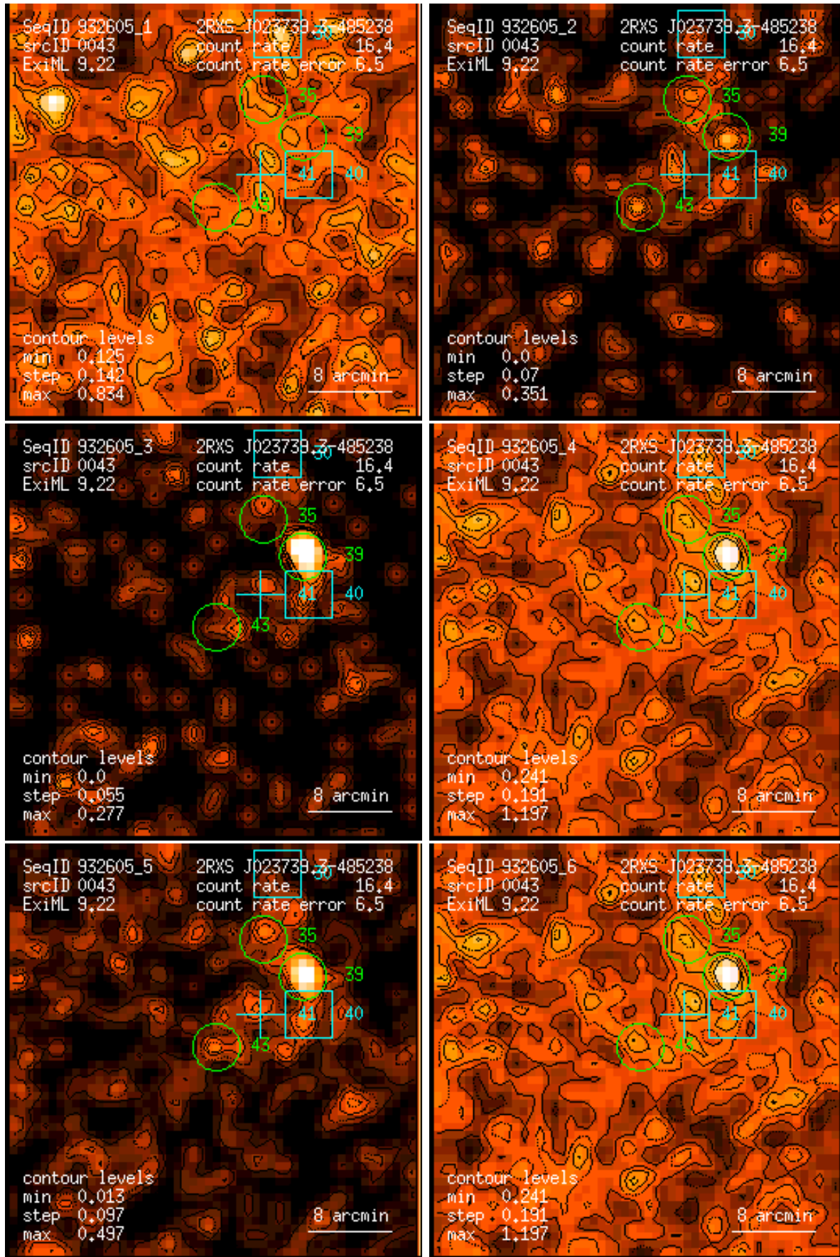
Figure 43: RASS 932605: detection 0043: band rate images, Gaussian filter: (1) PSPC channels 11 – 41, (2) 52 – 90, (3) 91 – 201, (4) 11 – 235, (5) 52 – 201, (6) 11 – 201. Broad band rates in counts/ks. Band rate contour levels in counts/ks/arcmin 2 .
