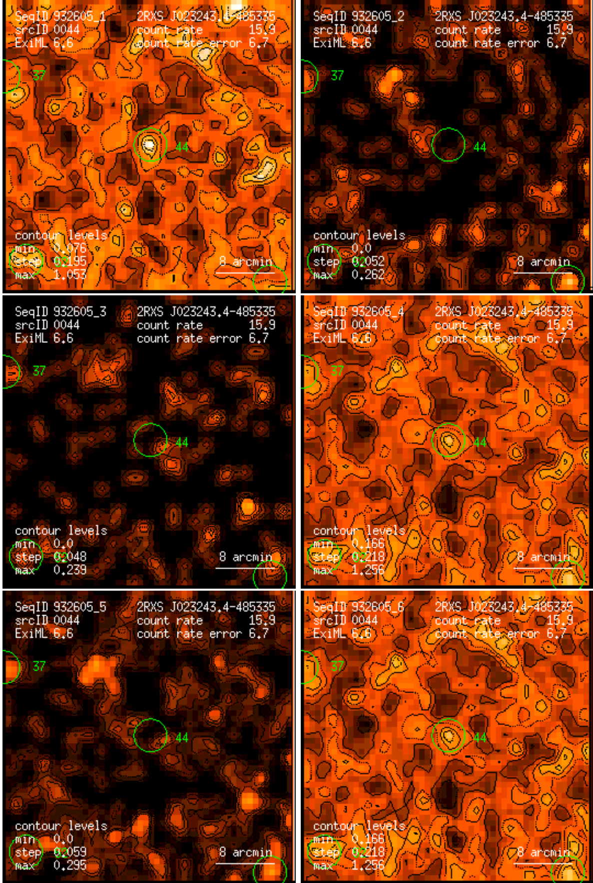
Figure 44: RASS 932605: detection 0044: band rate images, Gaussian filter: (1) PSPP channels 11 – 41, (2) 52 – 90, (3) 91 – 201, (4) 11 – 235, (5) 52 – 201, (6) 11 – 201. Broad band rates in counts/ks. Band rate contour levels in counts/ks/arcmin 2 .
