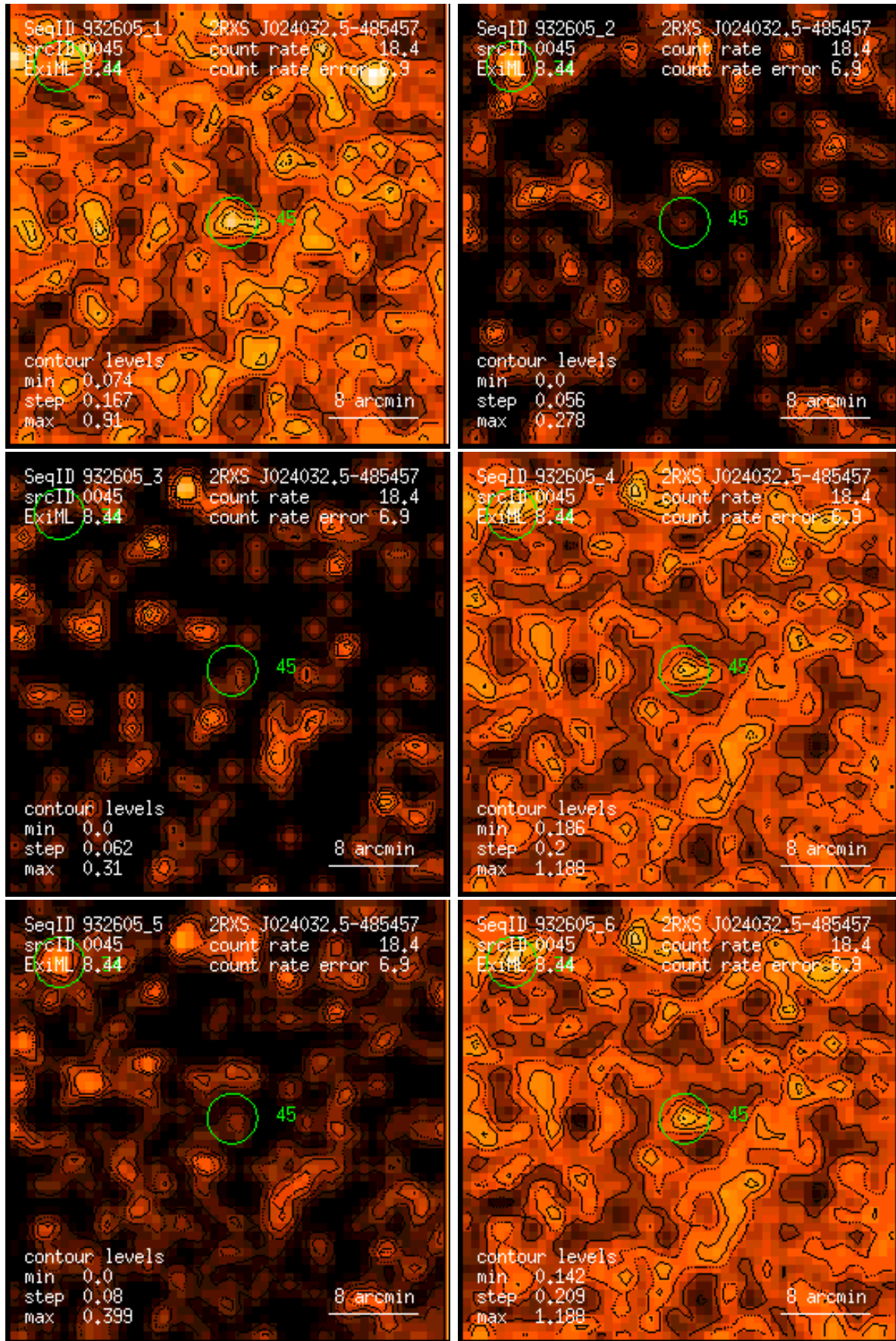
Figure 45: RASS 932605: detection 0045: band rate images, Gaussian filter: (1) PSPC channels 11 – 41, (2) 52 – 90, (3) 91 – 201, (4) 11 – 235, (5) 52 – 201, (6) 11 – 201. Broad band rates in counts/ks. Band rate contour levels in counts/ks/arcmin 2 .
