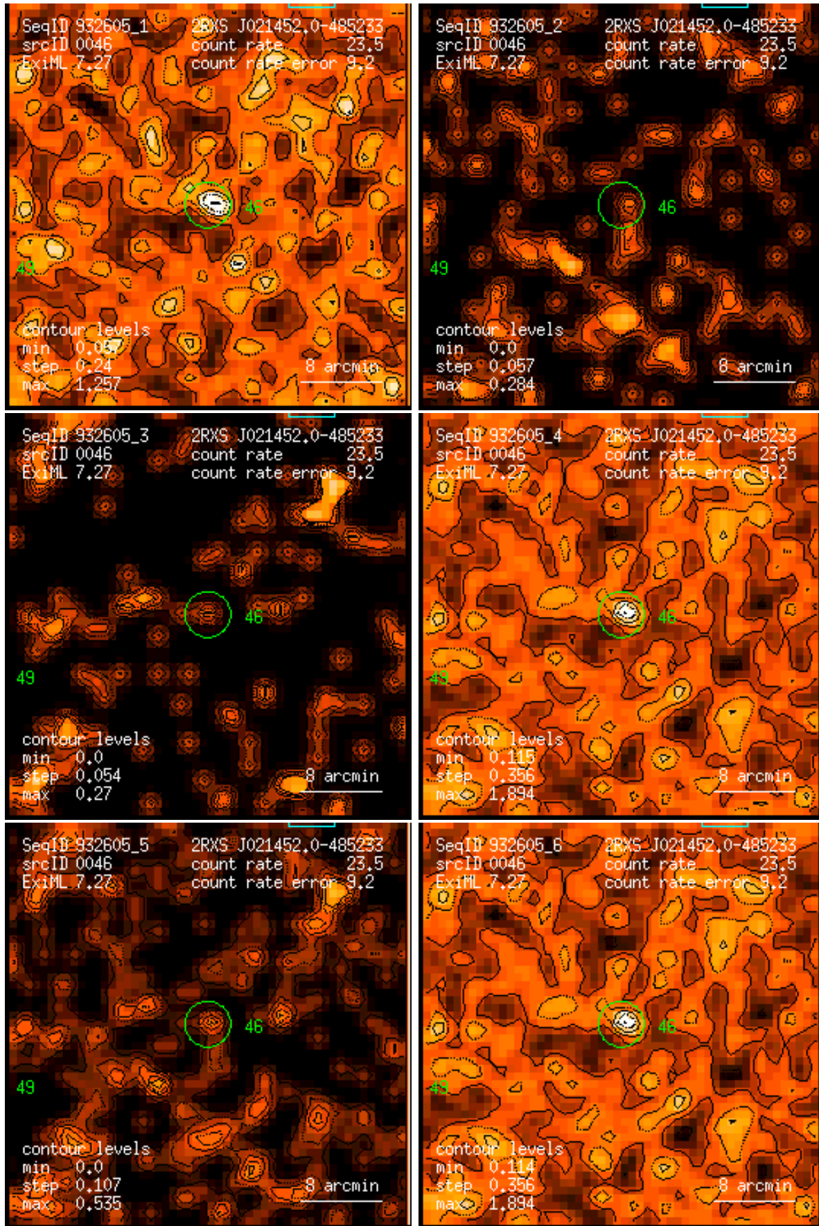
Figure 46: RASS 932605: detection 0046: band rate images, Gaussian filter: (1) PSPC channels 11 – 41, (2) 52 – 90, (3) 91 – 201, (4) 11 – 235, (5) 52 – 201, (6) 11 – 201. Broad band rates in counts/ks. Band rate contour levels in counts/ks/arcmin 2 .
