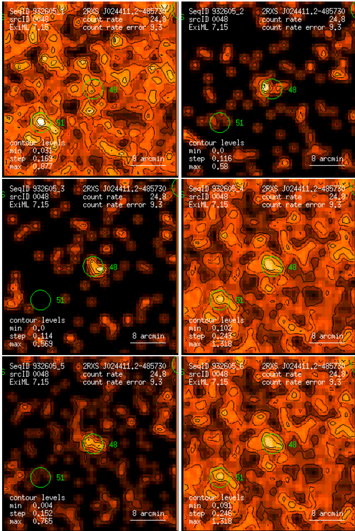
Figure 48: RASS 932605: detection 0048: band rate images, Gaussian filter: (1) PSPC channels 11 – 41, (2) 52 – 90, (3) 91 – 201, (4) 11 – 235, (5) 52 – 201, (6) 11 – 201. Broad band rates in counts/ks. Band rate contour levels in counts/ks/arcmin 2 .
