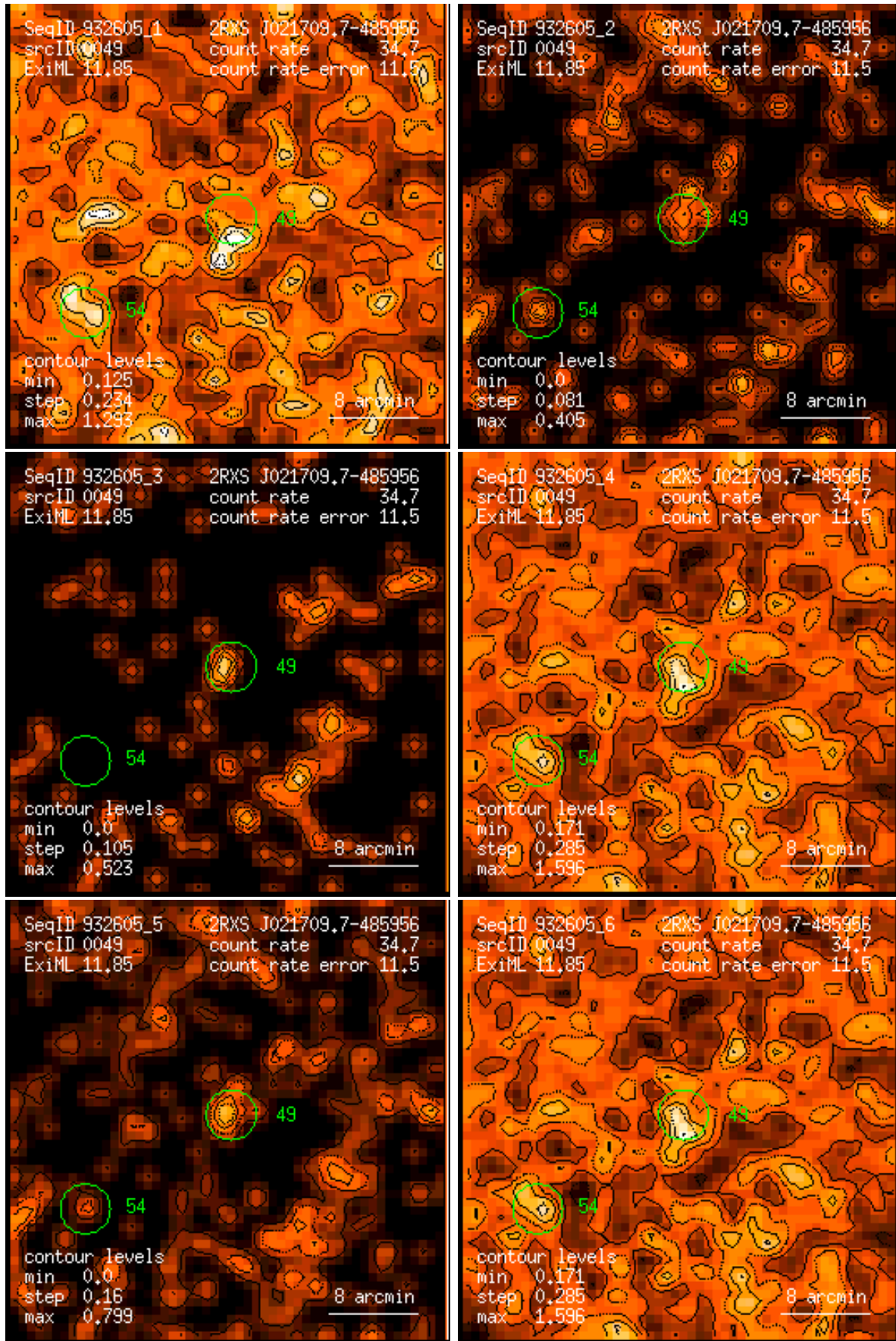
Figure 49: RASS 932605: detection 0049: band rate images, Gaussian filter: (1) PSPC channels 11 – 41, (2) 52 – 90, (3) 91 – 201, (4) 11 – 235, (5) 52 – 201, (6) 11 – 201. Broad band rates in counts/ks. Band rate contour levels in counts/ks/arcmin 2 .
