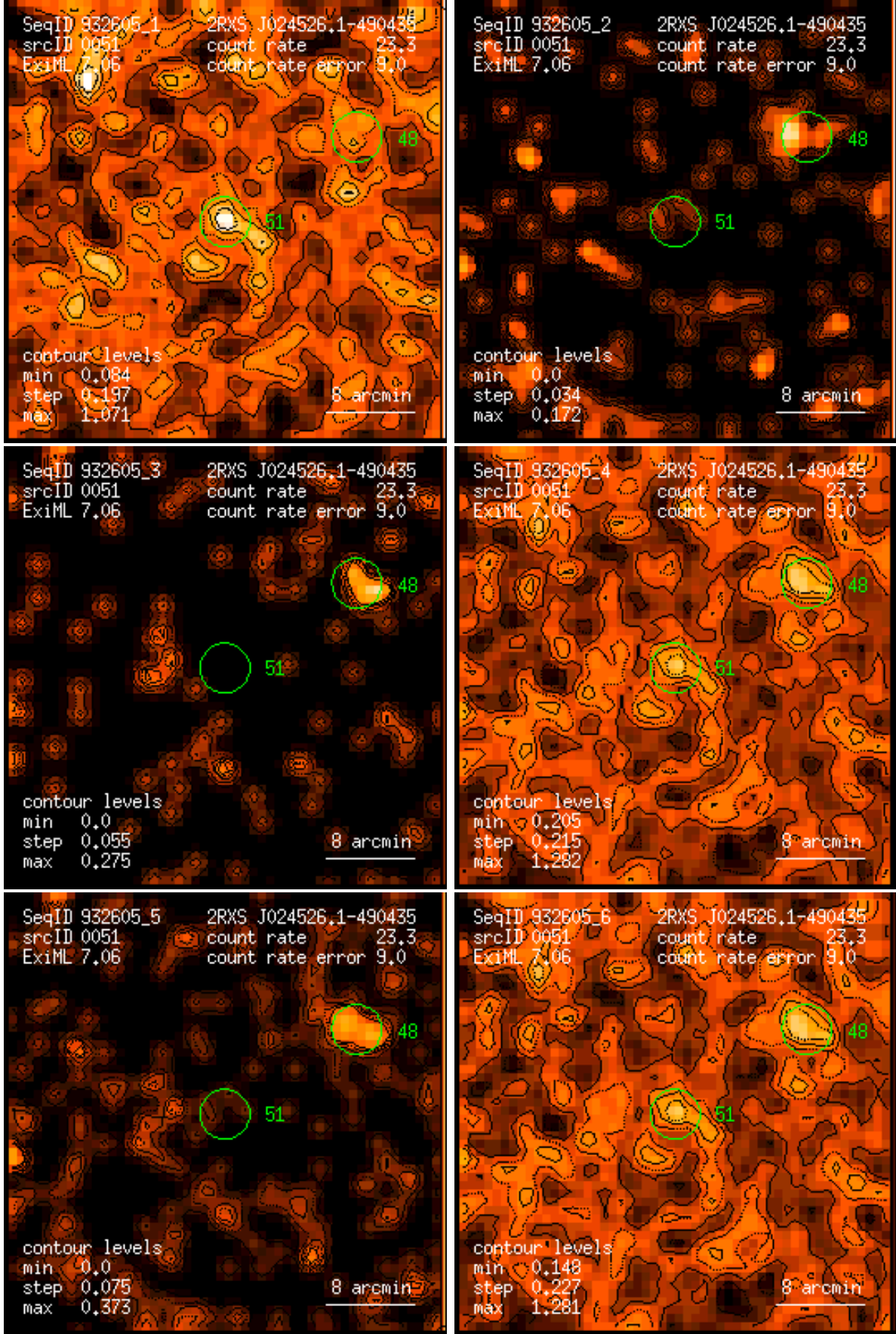
Figure 51: RASS 932605: detection 0051: band rate images, Gaussian filter: (1) PSPC channels 11 – 41, (2) 52 – 90, (3) 91 – 201, (4) 11 – 235, (5) 52 – 201, (6) 11 – 201. Broad band rates in counts/ks. Band rate contour levels in counts/ks/arcmin 2 .
