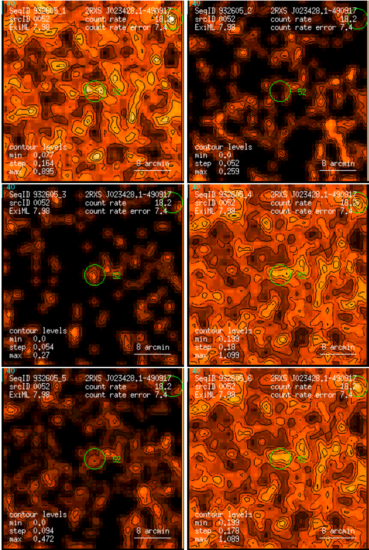
Figure 52: RASS 932605: detection 0052: band rate images, Gaussian filter: (1) PSPC channels 11 – 41, (2) 52 – 90, (3) 91 – 201, (4) 11 – 235, (5) 52 – 201, (6) 11 – 201. Broad band rates in counts/ks. Band rate contour levels in counts/ks/arcmin 2 .
