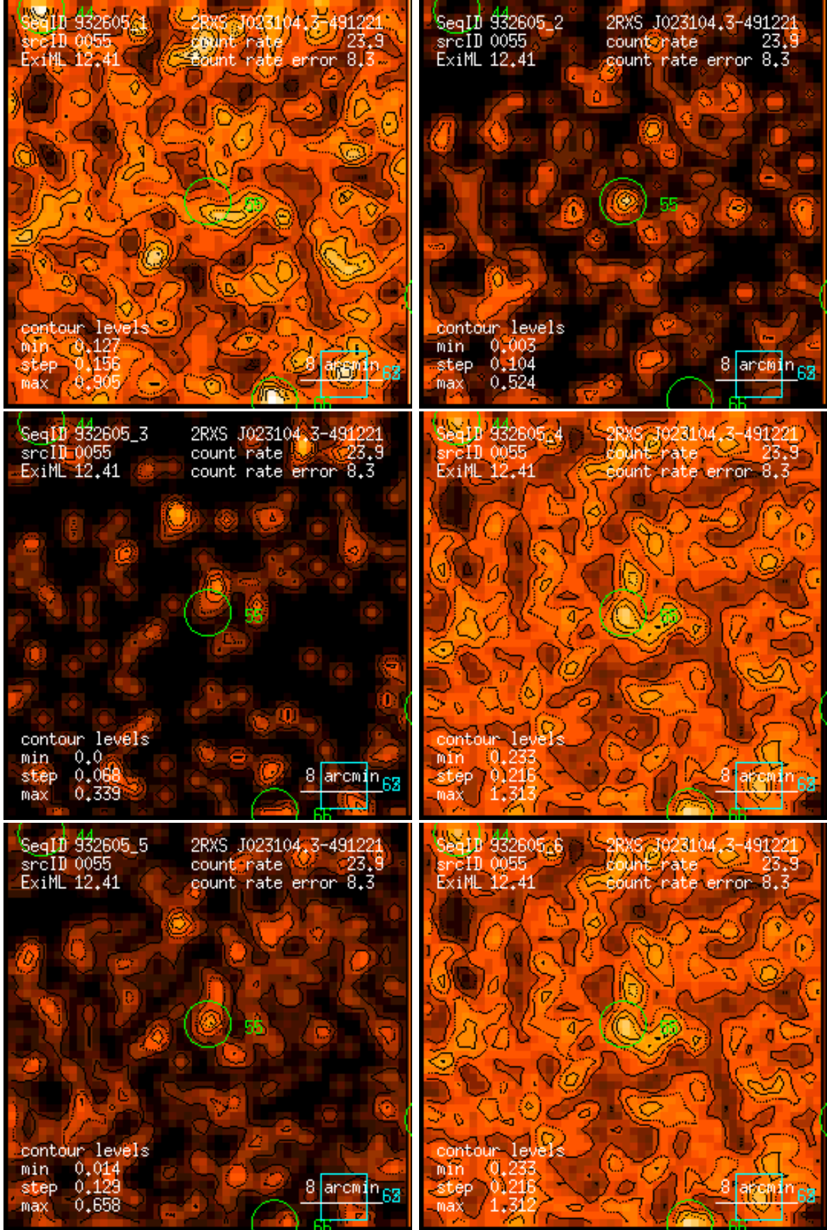
Figure 55: RASS 932605: detection 0055: band rate images, Gaussian filter: (1) PSPC channels 11 – 41, (2) 52 – 90, (3) 91 – 201, (4) 11 – 235, (5) 52 – 201, (6) 11 – 201. Broad band rates in counts/ks. Band rate contour levels in counts/ks/arcmin 2 .
