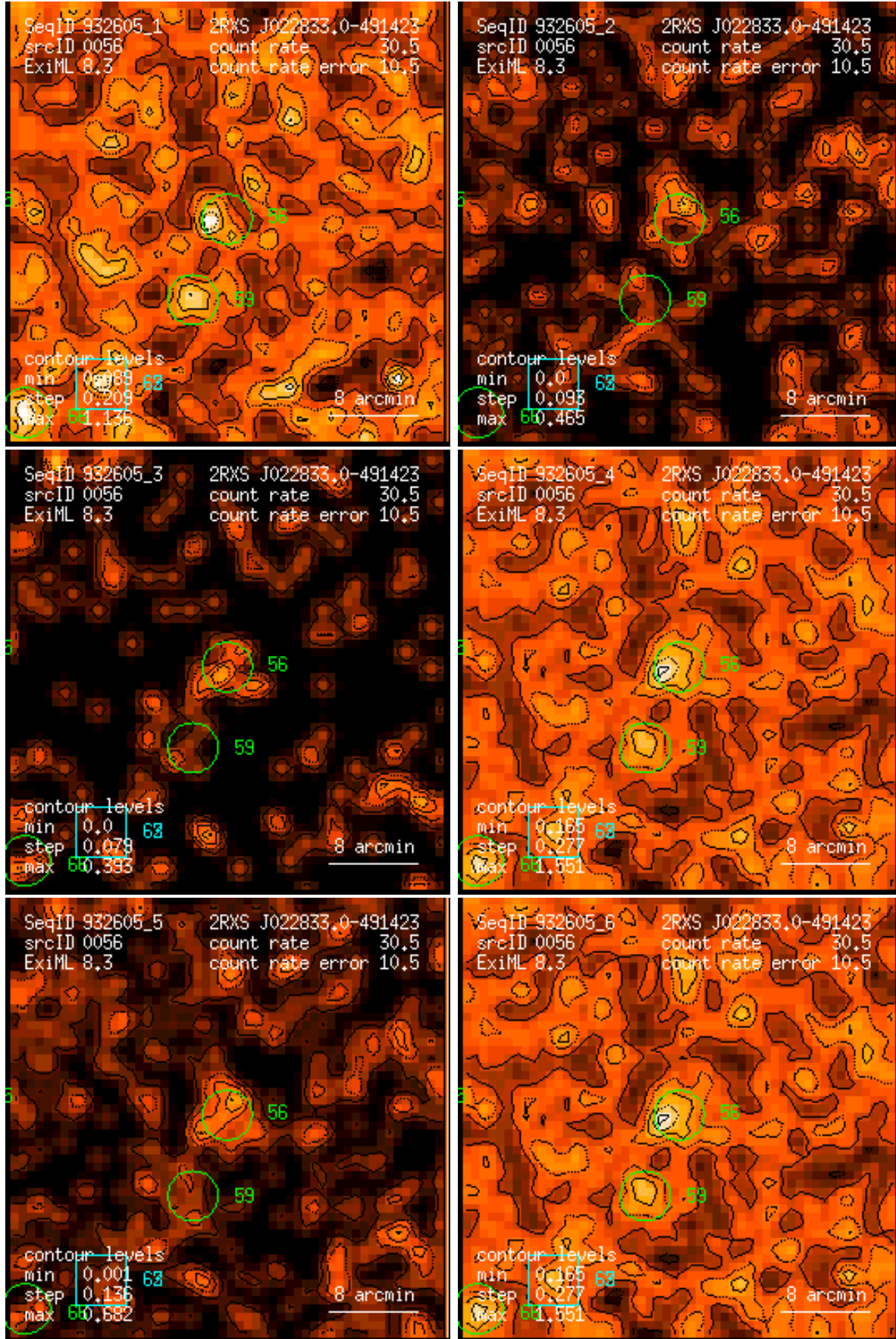
Figure 56: RASS 932605: detection 0056: band rate images, Gaussian filter: (1) PSPC channels 11 – 41, (2) 52 – 90, (3) 91 – 201, (4) 11 – 235, (5) 52 – 201, (6) 11 – 201. Broad band rates in counts/ks. Band rate contour levels in counts/ks/arcmin 2 .
