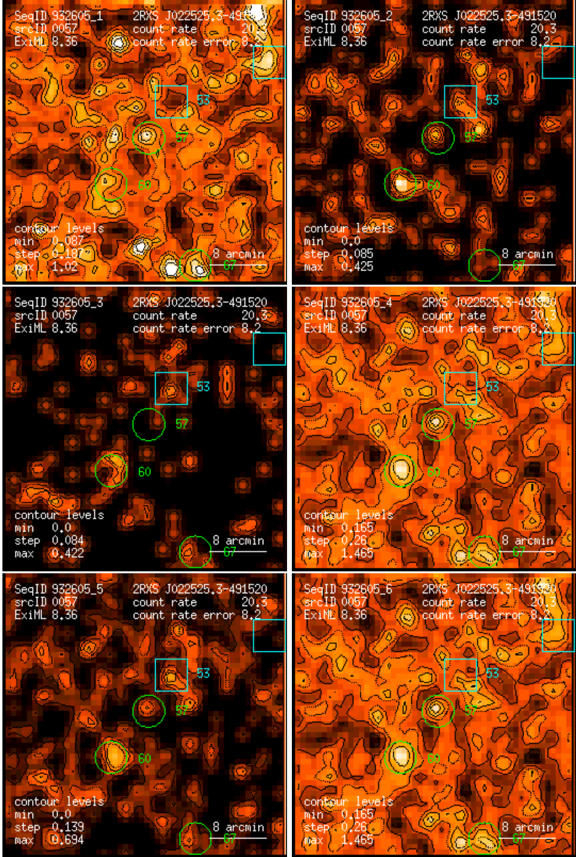
Figure 57: RASS 932605: detection 0057: band rate images, Gaussian filter: (1) PSPC channels 11 – 41, (2) 52 – 90, (3) 91 – 201, (4) 11 – 235, (5) 52 – 201, (6) 11 – 201. Broad band rates in counts/ks. Band rate contour levels in counts/ks/arcmin 2 .
