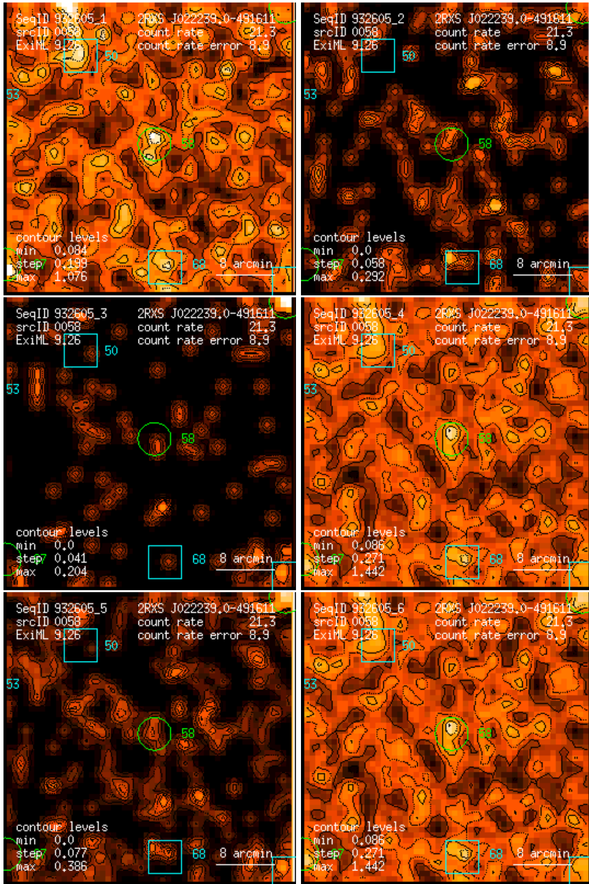
Figure 58: RASS 932605: detection 0058: band rate images, Gaussian filter: (1) PSPC channels 11 – 41, (2) 52 – 90, (3) 91 – 201, (4) 11 – 235, (5) 52 – 201, (6) 11 – 201. Broad band rates in counts/ks. Band rate contour levels in counts/ks/arcmin 2 .
