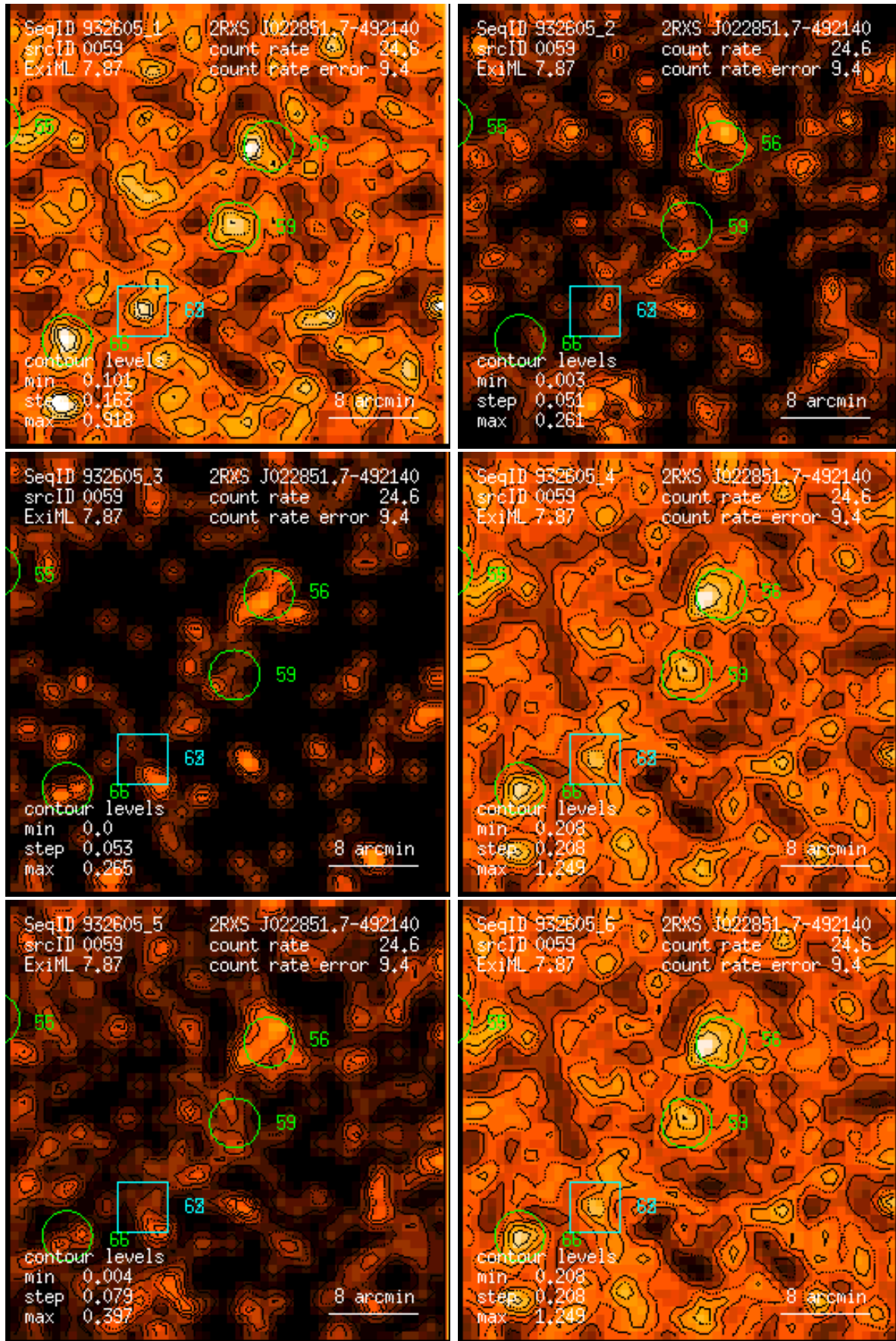
Figure 59: RASS 932605: detection 0059: band rate images, Gaussian filter: (1) PSPC channels 11 – 41, (2) 52 – 90, (3) 91 – 201, (4) 11 – 235, (5) 52 – 201, (6) 11 – 201. Broad band rates in counts/ks. Band rate contour levels in counts/ks/arcmin 2 .
