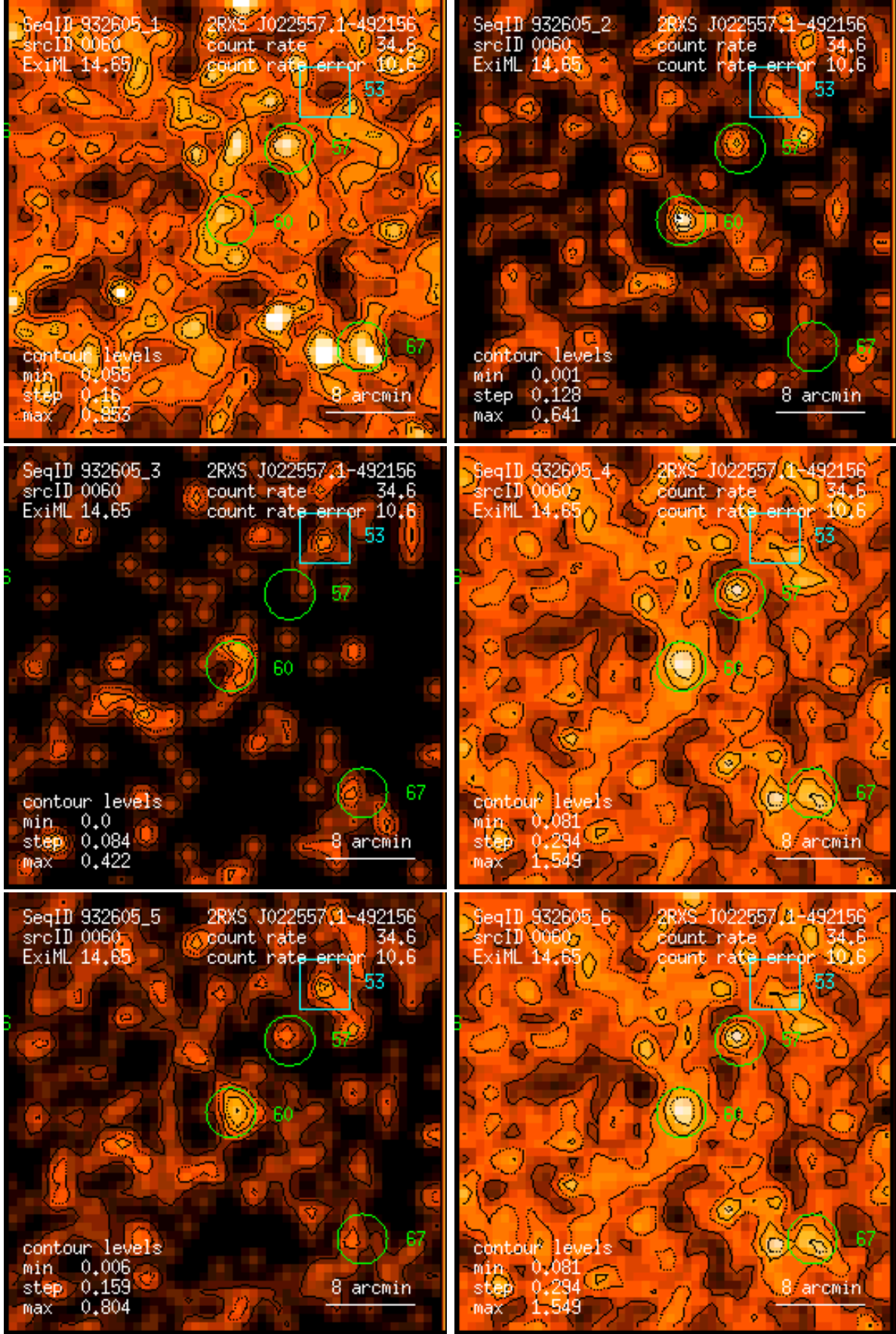
Figure 60: RASS 932605: detection 0060: band rate images, Gaussian filter: (1) PSPC channels 11 – 41, (2) 52 – 90, (3) 91 – 201, (4) 11 – 235, (5) 52 – 201, (6) 11 – 201. Broad band rates in counts/ks. Band rate contour levels in counts/ks/arcmin 2 .
