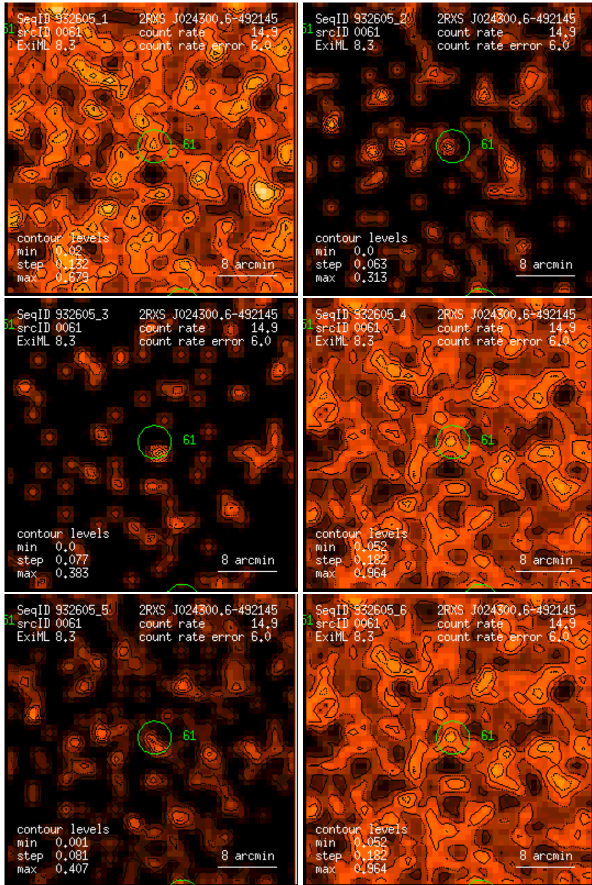
Figure 61: RASS 932605: detection 0061: band rate images, Gaussian filter: (1) PSPC channels 11 – 41, (2) 52 – 90, (3) 91 – 201, (4) 11 – 235, (5) 52 – 201, (6) 11 – 201. Broad band rates in counts/ks. Band rate contour levels in counts/ks/arcmin 2 .
