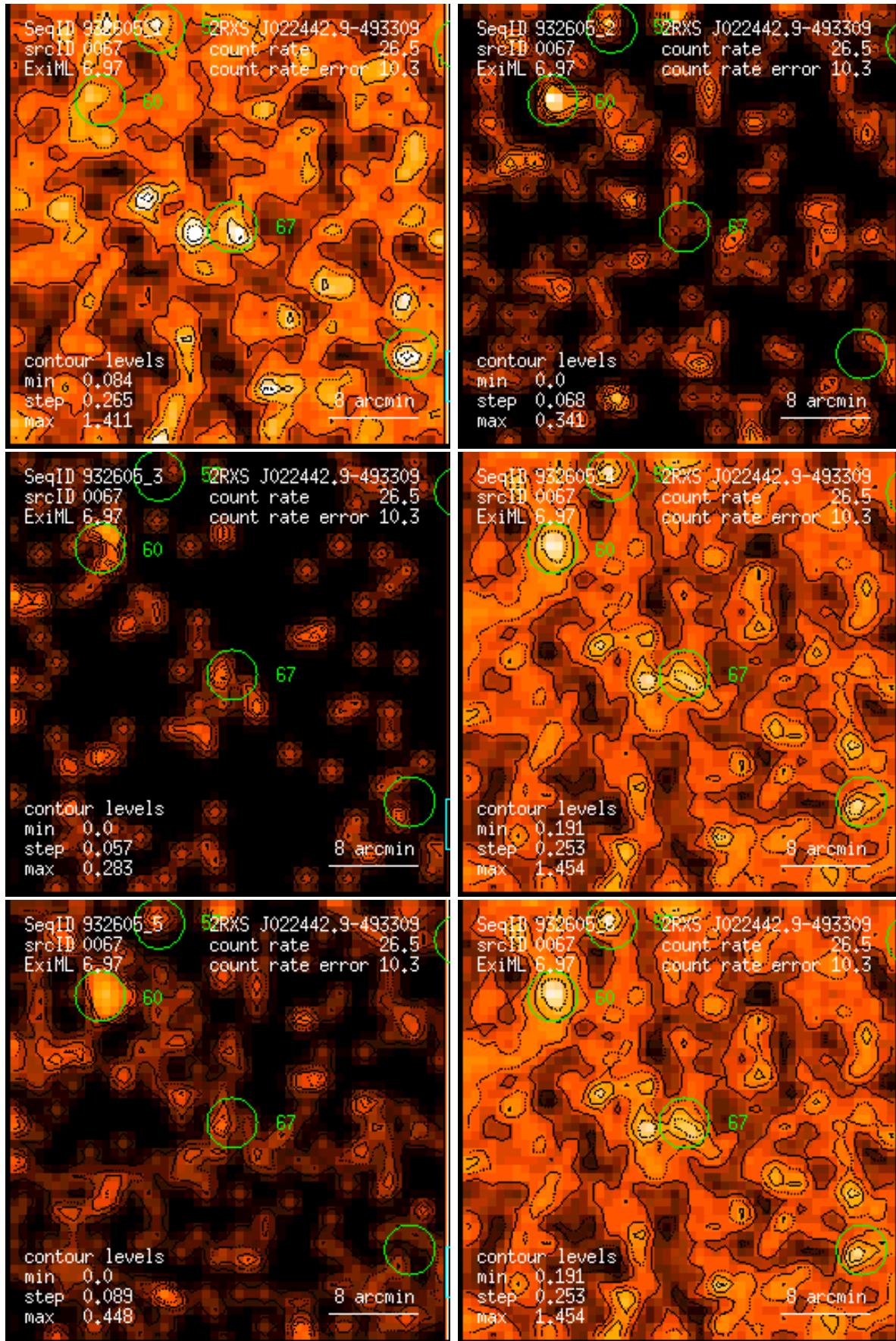
Figure 67: RASS 932605: detection 0067: band rate images, Gaussian filter: (1) PSPC channels 11 – 41, (2) 52 – 90, (3) 91 – 201, (4) 11 – 235, (5) 52 – 201, (6) 11 – 201. Broad band rates in counts/ks. Band rate contour levels in counts/ks/arcmin 2 .
