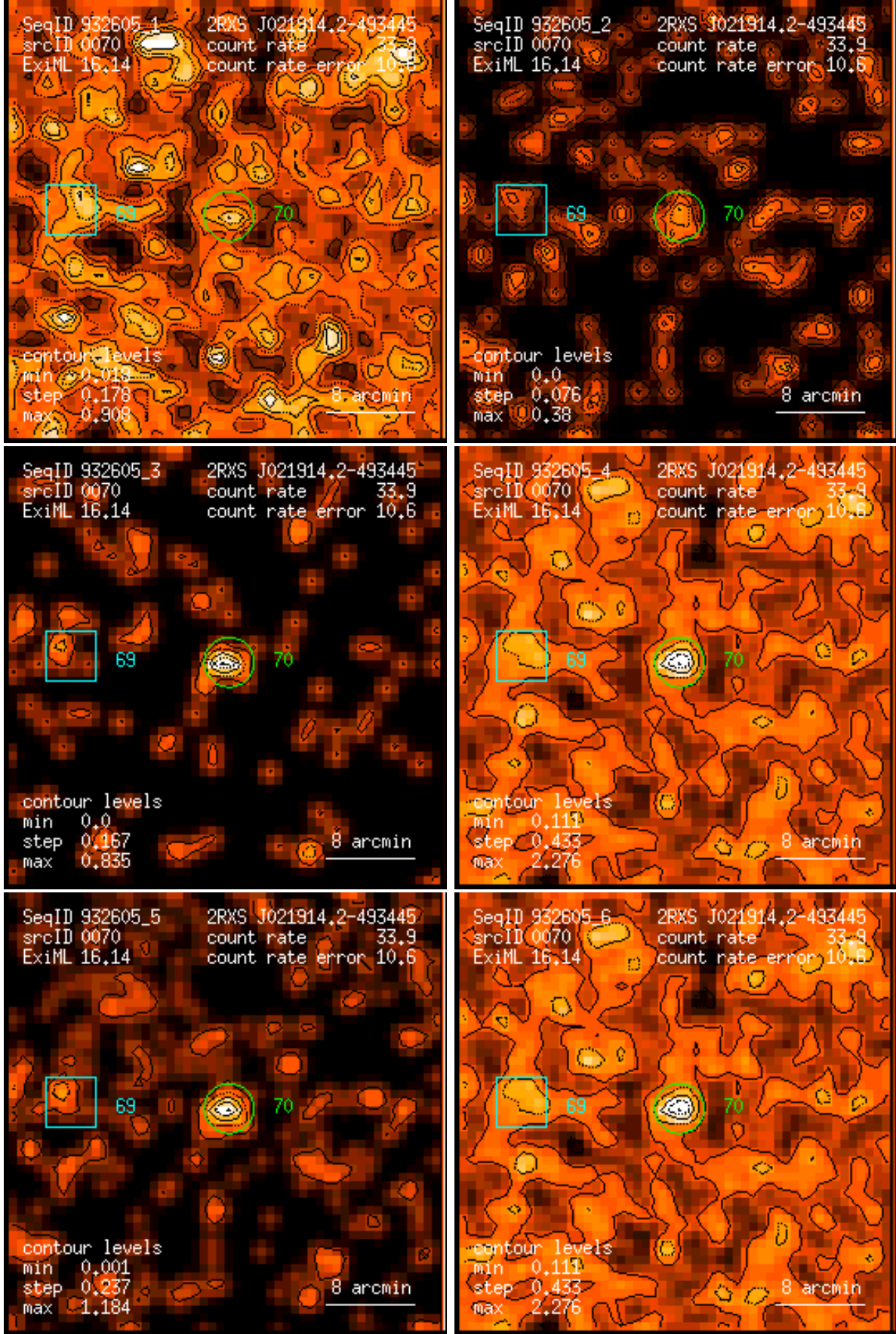
Figure 70: RASS 932605: detection 0070: band rate images, Gaussian filter: (1) PSPC channels 11 – 41, (2) 52 – 90, (3) 91 – 201, (4) 11 – 235, (5) 52 – 201, (6) 11 – 201. Broad band rates in counts/ks. Band rate contour levels in counts/ks/arcmin 2 .
