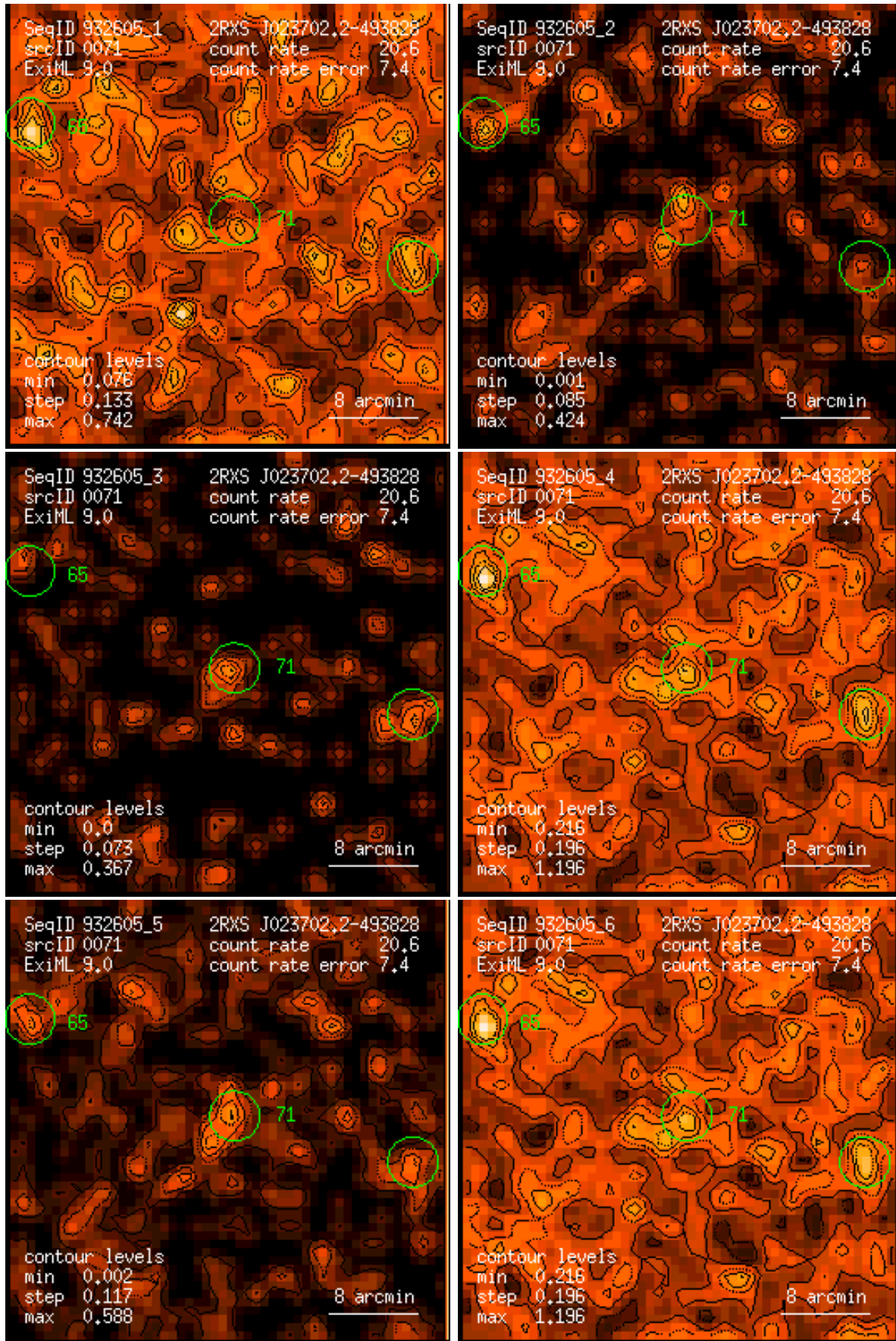
Figure 71: RASS 932605: detection 0071: band rate images, Gaussian filter: (1) PSPC channels 11 – 41, (2) 52 – 90, (3) 91 – 201, (4) 11 – 235, (5) 52 – 201, (6) 11 – 201. Broad band rates in counts/ks. Band rate contour levels in counts/ks/arcmin 2 .
