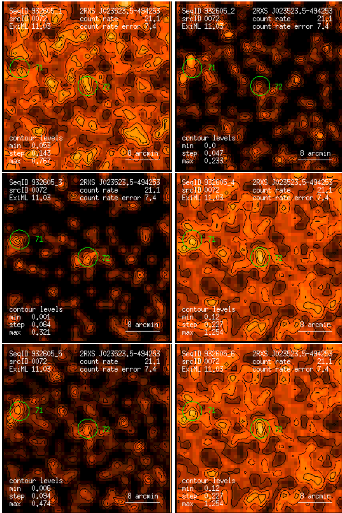
Figure 72: RASS 932605: detection 0072: band rate images, Gaussian filter: (1) PSPC channels 11 – 41, (2) 52 – 90, (3) 91 – 201, (4) 11 – 235, (5) 52 – 201, (6) 11 – 201. Broad band rates in counts/ks. Band rate contour levels in counts/ks/arcmin 2 .
