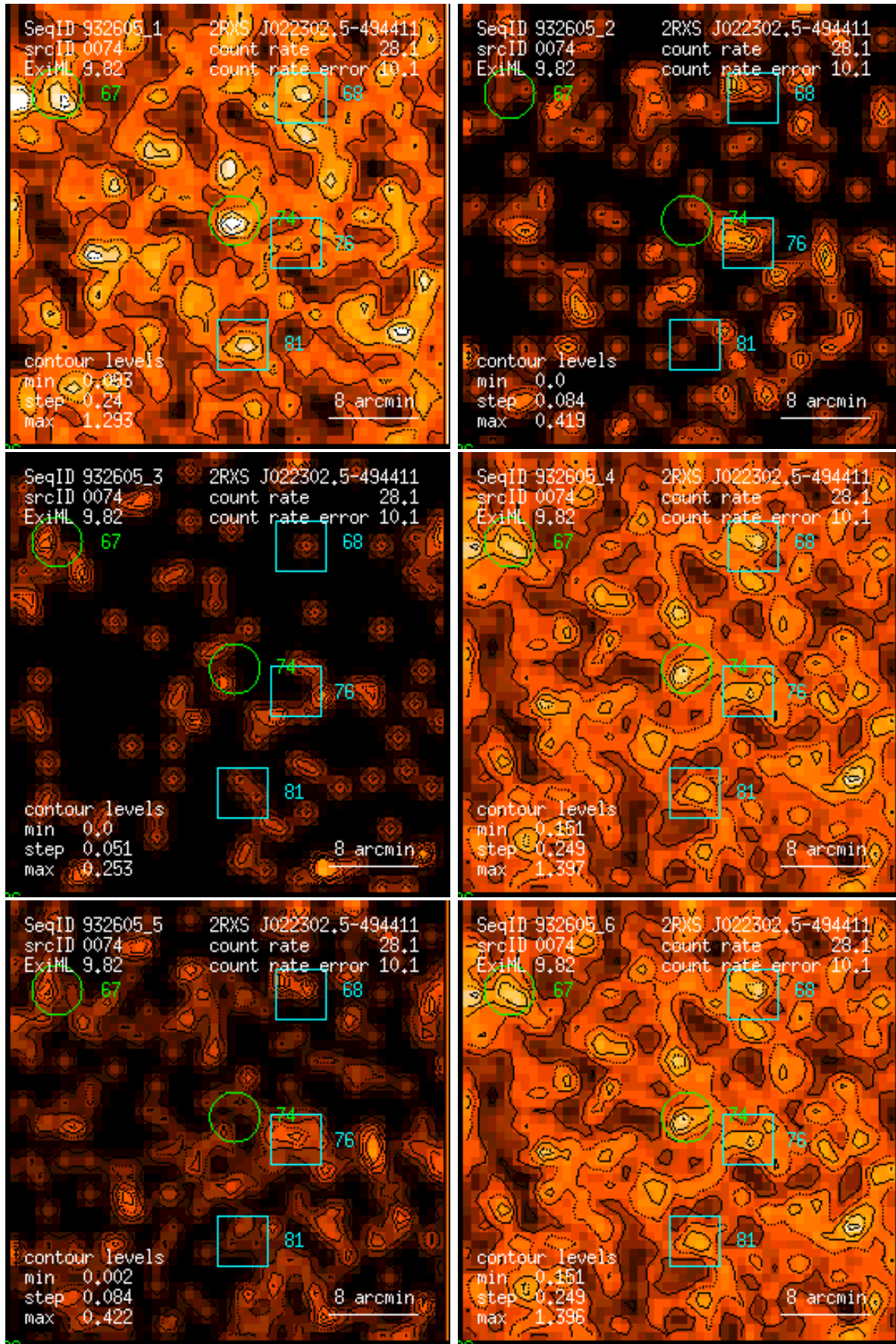
Figure 74: RASS 932605: detection 0074: band rate images, Gaussian filter: (1) PSPC channels 11 – 41, (2) 52 – 90, (3) 91 – 201, (4) 11 – 235, (5) 52 – 201, (6) 11 – 201. Broad band rates in counts/ks. Band rate contour levels in counts/ks/arcmin 2 .
