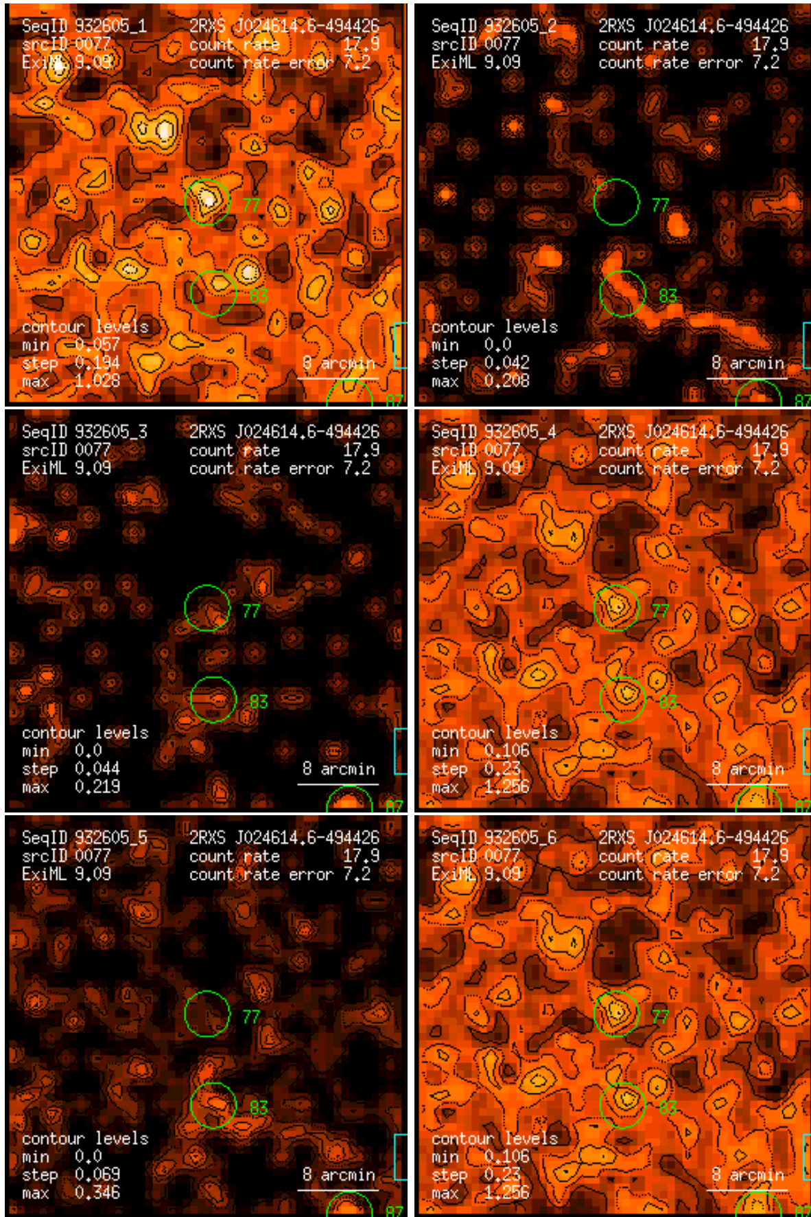
Figure 77: RASS 932605: detection 0077: band rate images, Gaussian filter: (1) PSPC channels 11 – 41, (2) 52 – 90, (3) 91 – 201, (4) 11 – 235, (5) 52 – 201, (6) 11 – 201. Broad band rates in counts/ks. Band rate contour levels in counts/ks/arcmin 2 .
