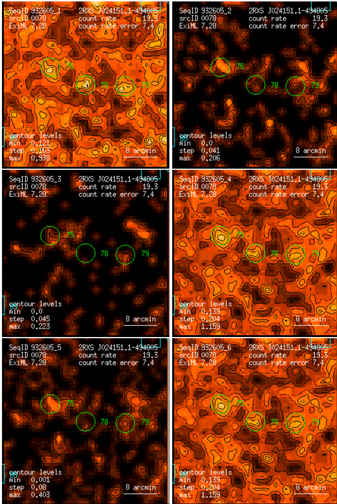
Figure 78: RASS 932605: detection 0078: band rate images, Gaussian filter: (1) PSPC channels 11 – 41, (2) 52 – 90, (3) 91 – 201, (4) 11 – 235, (5) 52 – 201, (6) 11 – 201. Broad band rates in counts/ks. Band rate contour levels in counts/ks/arcmin 2 .
