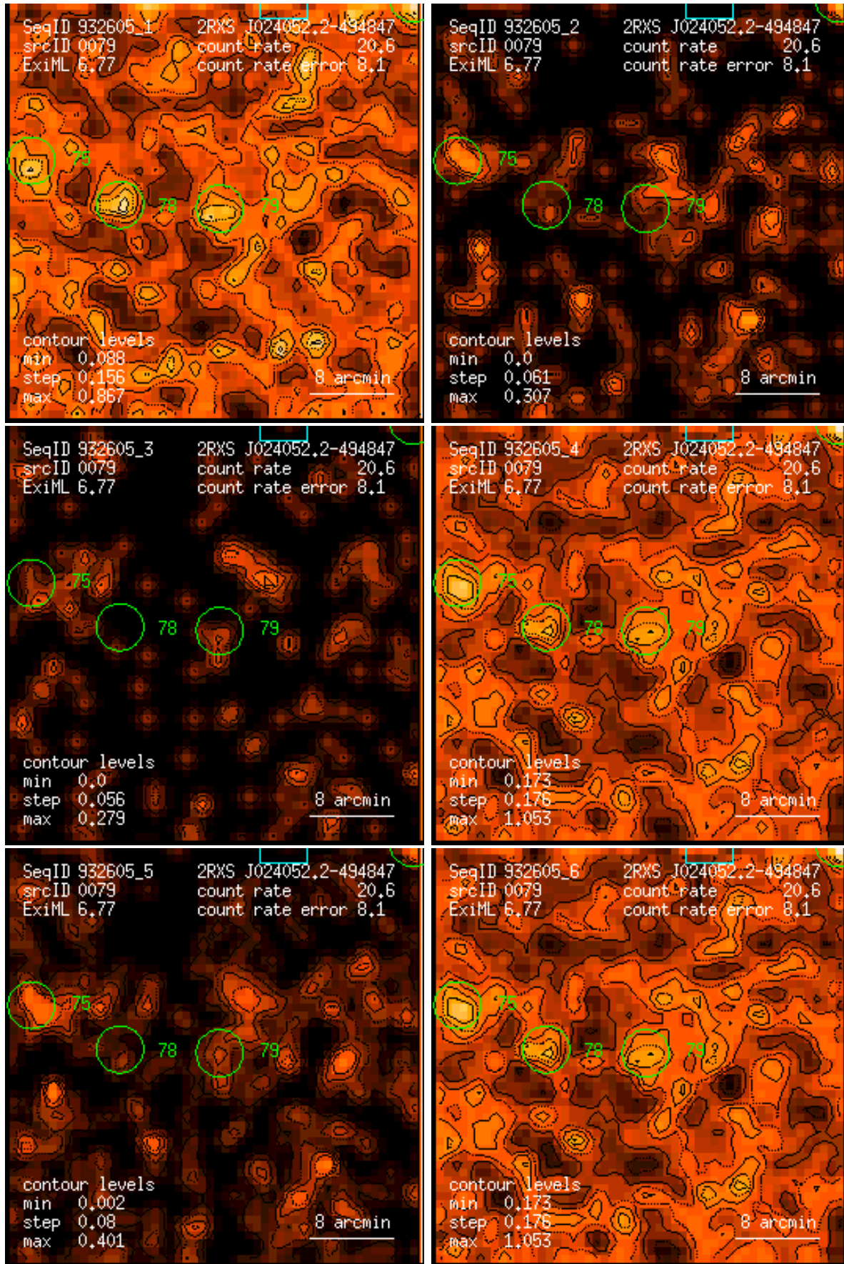
Figure 79: RASS 932605: detection 0079: band rate images, Gaussian filter: (1) PSPC channels 11 – 41, (2) 52 – 90, (3) 91 – 201, (4) 11 – 235, (5) 52 – 201, (6) 11 – 201. Broad band rates in counts/ks. Band rate contour levels in counts/ks/arcmin 2 .
