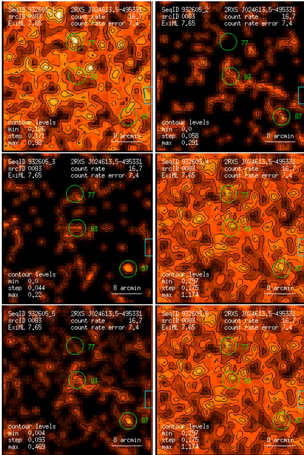
Figure 83: RASS 932605: detection 0083: band rate images, Gaussian filter: (1) PSPC channels 11 – 41, (2) 52 – 90, (3) 91 – 201, (4) 11 – 235, (5) 52 – 201, (6) 11 – 201. Broad band rates in counts/ks. Band rate contour levels in counts/ks/arcmin 2 .
