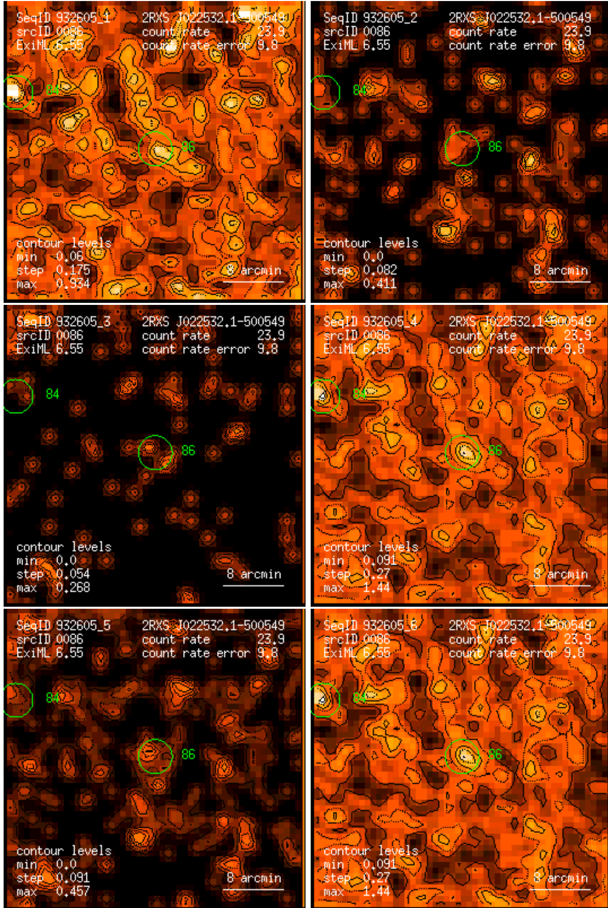
Figure 86: RASS 932605: detection 0086: band rate images, Gaussian filter: (1) PSPC channels 11 – 41, (2) 52 – 90, (3) 91 – 201, (4) 11 – 235, (5) 52 – 201, (6) 11 – 201. Broad band rates in counts/ks. Band rate contour levels in counts/ks/arcmin 2 .
