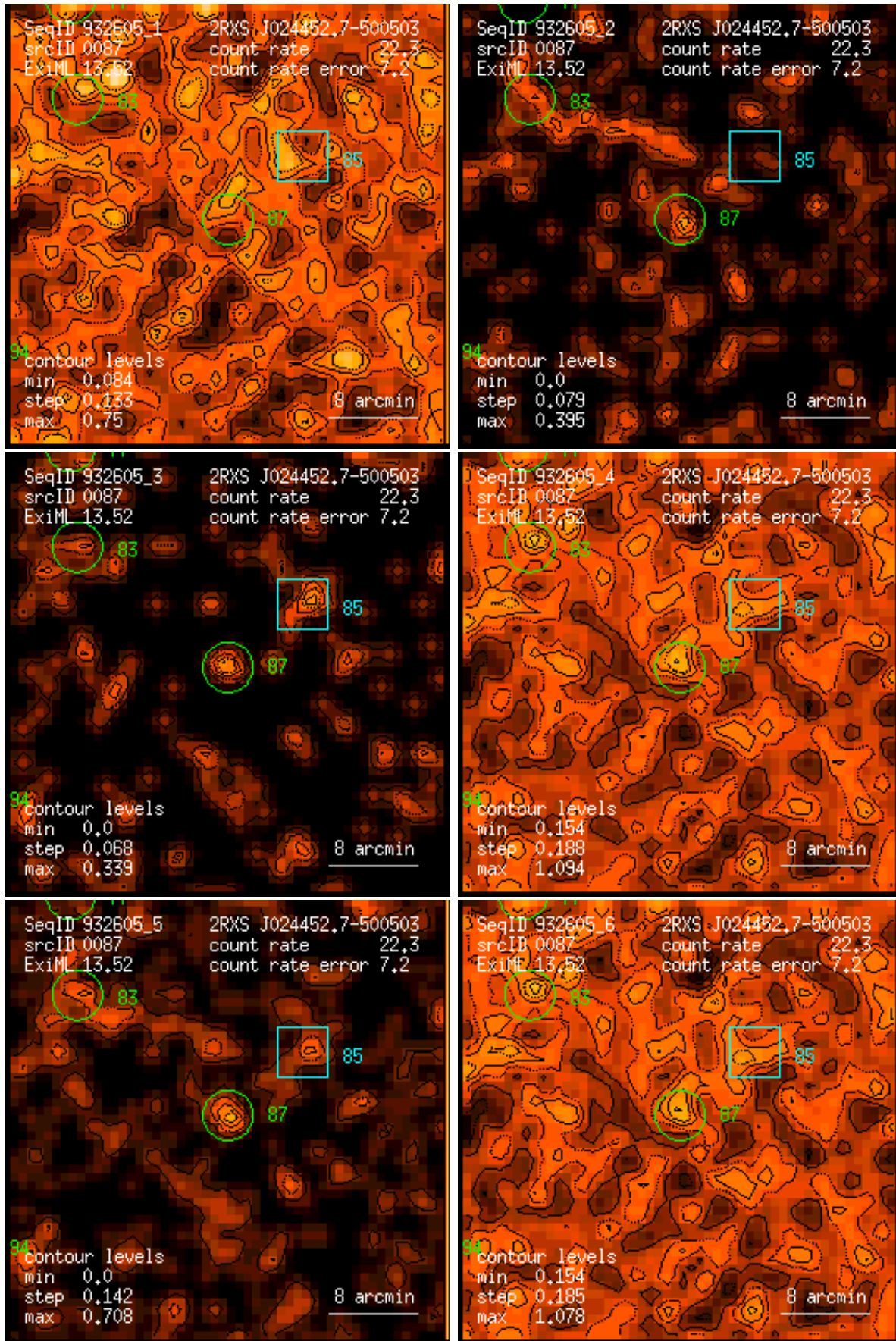
Figure 87: RASS 932605: detection 0087: band rate images, Gaussian filter: (1) PSPC channels 11 – 41, (2) 52 – 90, (3) 91 – 201, (4) 11 – 235, (5) 52 – 201, (6) 11 – 201. Broad band rates in counts/ks. Band rate contour levels in counts/ks/arcmin 2 .
