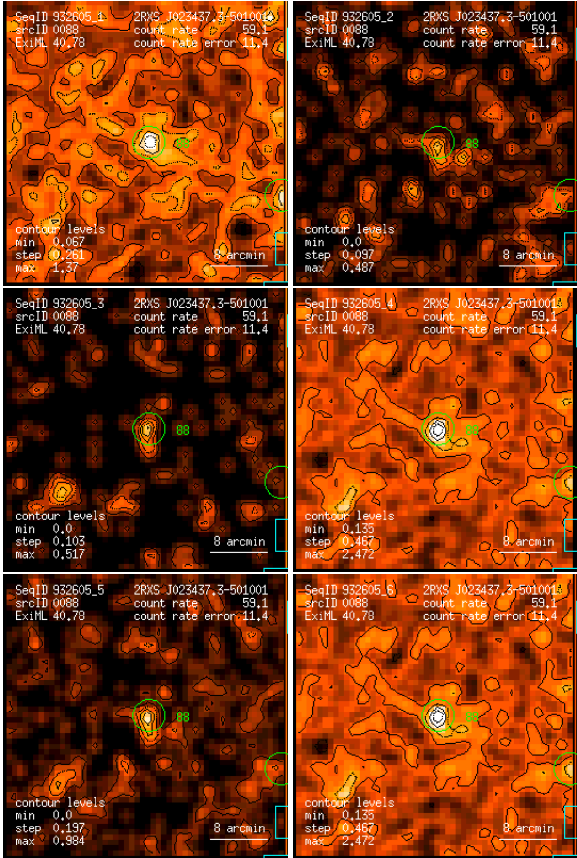
Figure 88: RASS 932605: detection 0088: band rate images, Gaussian filter: (1) PSPC channels 11 – 41, (2) 52 – 90, (3) 91 – 201, (4) 11 – 235, (5) 52 – 201, (6) 11 – 201. Broad band rates in counts/ks. Band rate contour levels in counts/ks/arcmin 2 .
