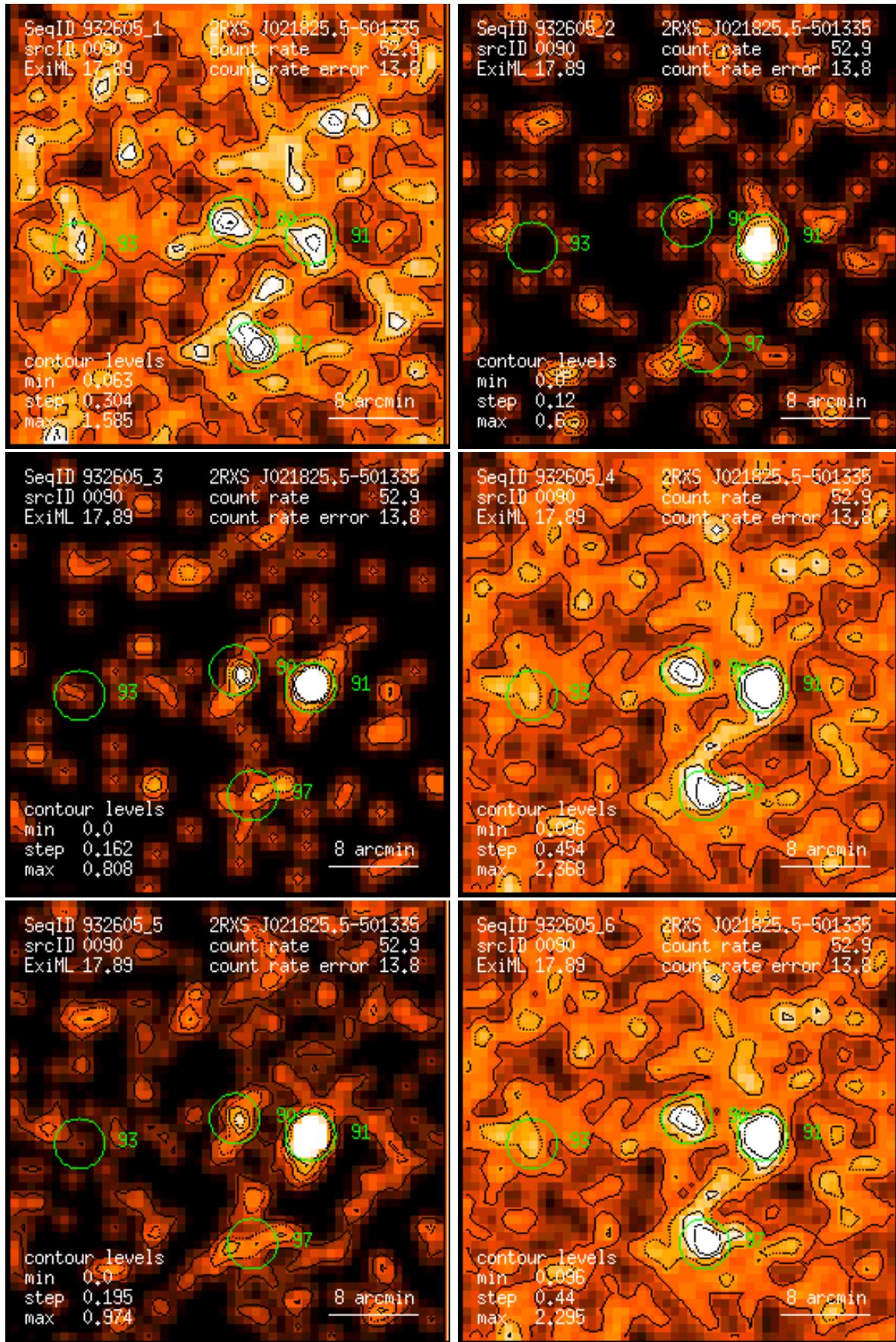
Figure 90: RASS 932605: detection 0090: band rate images, Gaussian filter: (1) PSPC channels 11 – 41, (2) 52 – 90, (3) 91 – 201, (4) 11 – 235, (5) 52 – 201, (6) 11 – 201. Broad band rates in counts/ks. Band rate contour levels in counts/ks/arcmin 2 .
