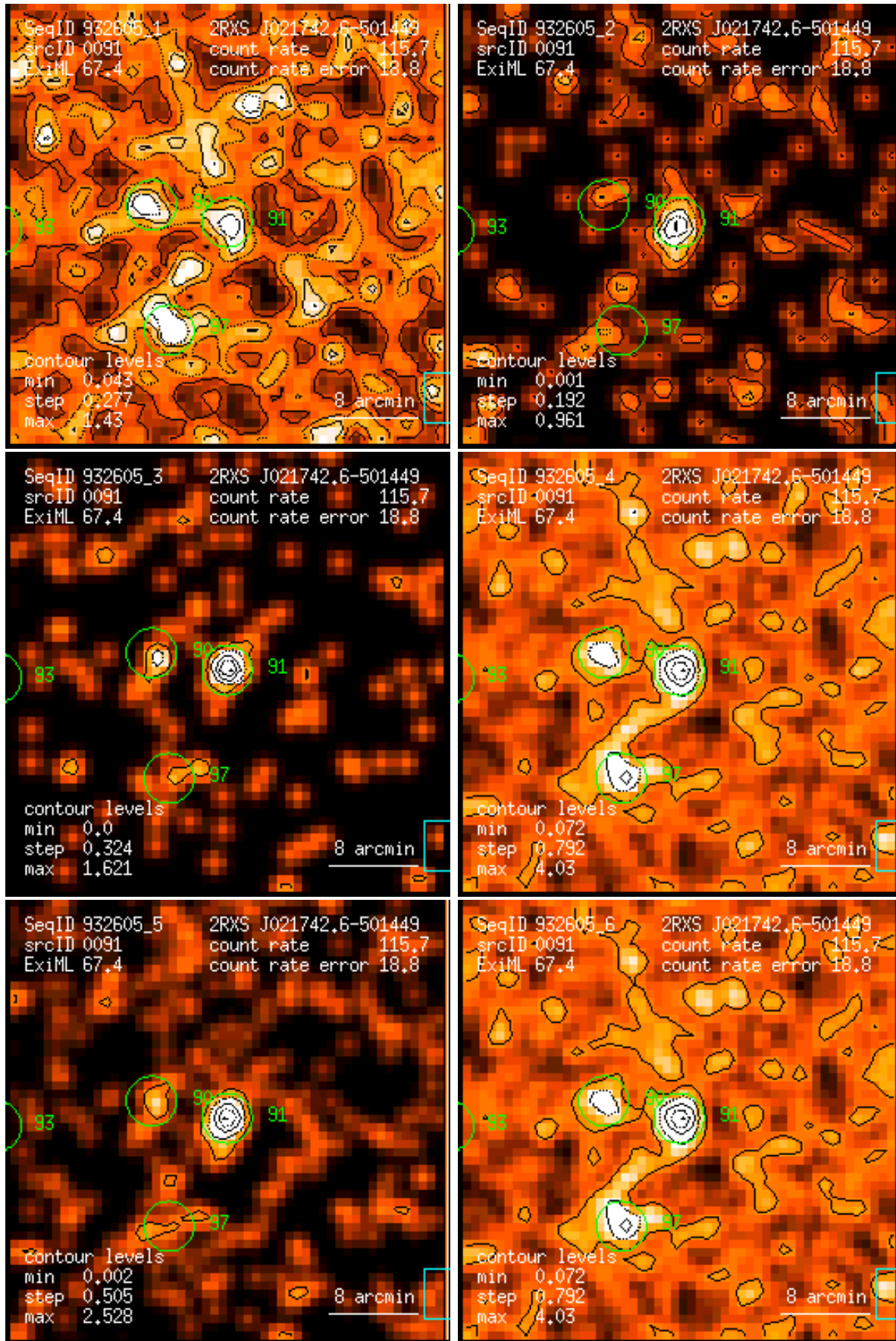
Figure 91: RASS 932605: detection 0091: band rate images, Gaussian filter: (1) PSPC channels 11 – 41, (2) 52 – 90, (3) 91 – 201, (4) 11 – 235, (5) 52 – 201, (6) 11 – 201. Broad band rates in counts/ks. Band rate contour levels in counts/ks/arcmin 2 .
