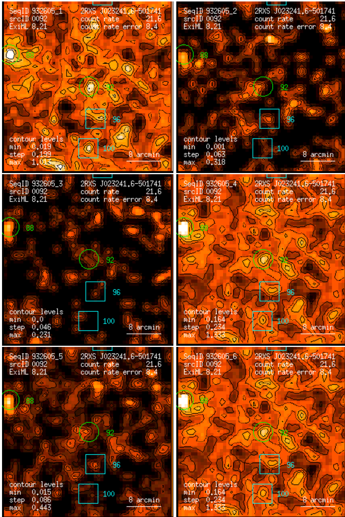
Figure 92: RASS 932605: detection 0092: band rate images, Gaussian filter: (1) PSPC channels 11 – 41, (2) 52 – 90, (3) 91 – 201, (4) 11 – 235, (5) 52 – 201, (6) 11 – 201. Broad band rates in counts/ks. Band rate contour levels in counts/ks/arcmin 2 .
